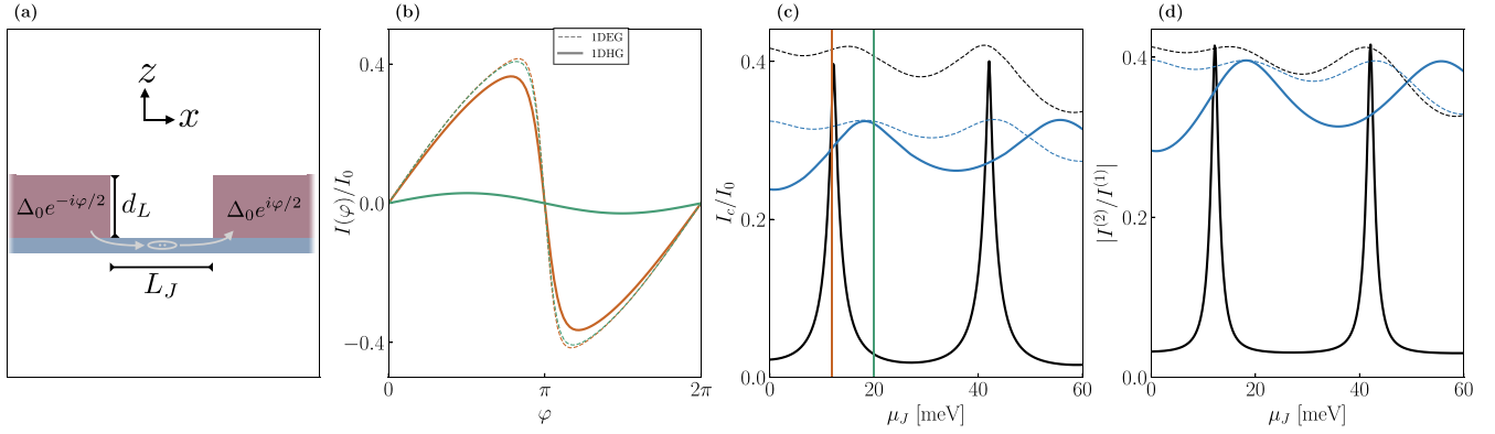
FIG. 3. One-dimensional JJ consisting of an infinite 1D semiconducting wire (blue), with a single subband that extends through both the junction region and the leads. Each lead is covered by a semi-infinite SC film (brown) with a phase difference \varphi across the JJ that generates a supercurrent I(\varphi) in the wire. When the leads are in the insulating regime (black lines), the critical current I_c [panel (c)] and the ratio between the first two harmonics of the CPR, |I^{(2)}/I^{(1)}| , [panel (d)] are strongly nonmonotonic: Adjusting the chemical potential \mu_J in the junction reveals sharp peaks in I_c and |I^{(2)}/I^{(1)}| [see panels (c) and (d)], corresponding to bound states confined around the normal junction region. In contrast, for a 1DEG coupled to a superconductor [dashed lines in panels (c) and (d)] or when the 1DHG is in the SC phase [blue lines in panels (c) and (d)], the system exhibits a more steady dependence of I_c and |I^{(2)}/I^{(1)}| on \mu_J . In these cases, the oscillations are due to Andreev bound states whose transmissivity is \mu_J dependent. The vertical lines in panel (c) show \mu_J for the CPRs I(\varphi) in panel (b) [ \mu_J = 12 meV (orange) and 20 meV (green)]. The junction length is L_J = 50 nm, the superconductor thickness d_L = 20 nm, and the lattice constant a = 0.5 nm. Here, k_B T = \Delta_0/20 \approx 100 mK, \mu_{sm} = 90 meV, and the hopping between the semiconductor and superconductor t_c = 50 meV (see Appendix D). For the black lines in panels (c) and (d) and all CPRs in panel (b) \mu_{sc} \approx 293 meV, while for the blue lines in panels (c) and (d) \mu_{sc} \approx 306 meV. The effective masses are the same as in Fig. 1. The supercurrents are normalized relative to I_0 = |e|\Delta_0 \approx 49 nA.
