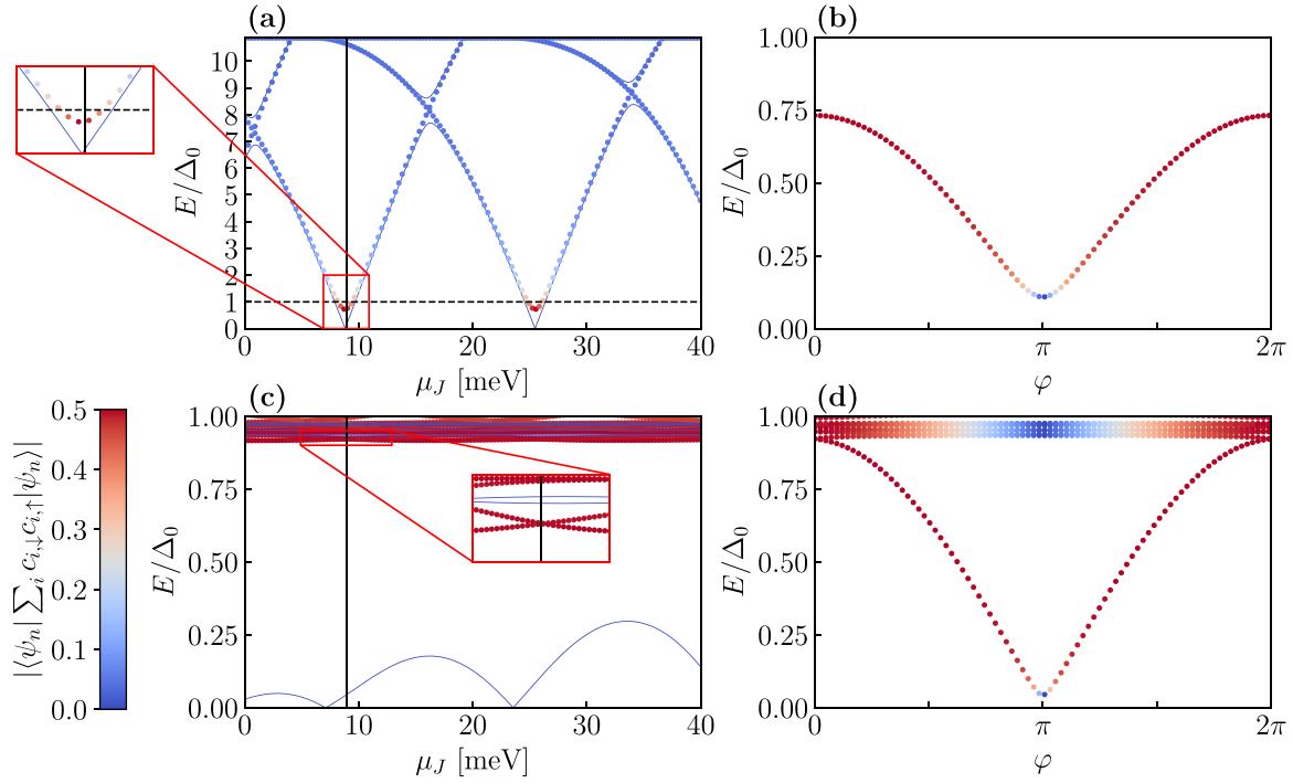
FIG. 8. Plots of bound state energies for a JJ vs chemical potential \mu_J and superconducting phase \phi for 1DHG [panels (a) and (b)] and 1DEG [panels (c) and (d)]. The bound states for a 1DHG are localized in the normal section of the JJ due to the insulating gaps in the leads and carry significant SC correlations only when their energies are below \Delta_0 [which is indicated by the horizontal black dashed line in panel (a)]. (c) On the other hand, the ABSs that arise when the system is in the SC phase have a weaker dependence on \mu_J , both in their energies and in the SC correlation. The dotted lines in panels (a) and (c) are for \phi = 0 , where the SC correlation is maximal, whereas the full lines (blue) are for \phi = \pi , where the SC correlation is zero (in this case the pairing is \Delta_0 in the left lead and -\Delta_0 in the right lead). In panel (b), we show the energy of the lowest bound state as function of \phi for the leads being in the insulating phase at \mu_J = 8.9 meV [see vertical black line in panel (a)]. There are no states with energies just below the superconducting gap as well as there are no other states within the insulating gap, as can be seen in panel (a). For comparison, in panel (d), we show the energy-phase relation for the lowest n = 12 states for a 1DEG JJ with leads being in the SC proximity phase. Here, the ABS energy is around \Delta_0 for \phi close to zero and it almost merges with the bulk states. This is a reason why we included \phi = \pi in panel (c) to show the presence of the ABSs in the spectrum. The results are obtained from a finite-size system, with a single SC subband, described in Eqs. (D1) and (D2) with d_L = 2a . We used the following parameters: L = 3500 nm (total length of chain), L_J = 62 nm, a = 1 nm, t_{sm} = \pm 580 meV, t_{sc} = 36.2 meV, t_c = 5 meV, \mu_{sm} = 40 meV, \bar{\mu}_{sc} = 2.5 meV, and \Delta_0 = 0.2 meV. In panels (a) and (b), the effective masses have opposite signs, whereas in panels (c) and (d) they have the same signs.
