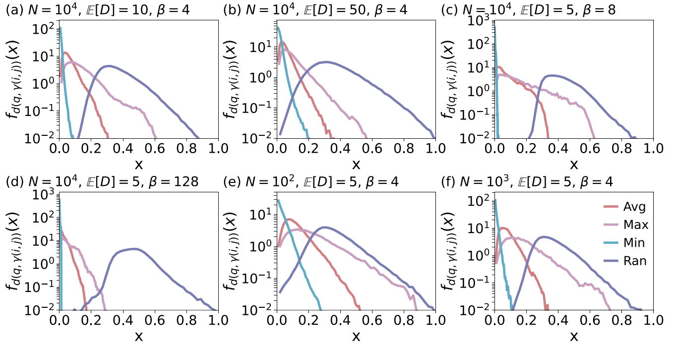
FIG. 8. The distribution of the average (avg), maximum (max), and minimum (min) distances between shortest path nodes and geodesics connecting shortest path end points. For comparison, we also plot the distribution of distances to geodesic from randomly selected nodes (ran). The distributions in panels (a)–(d) are obtained for a single SRGG realization and 10^6 random shortest paths. For panels (e) and (f), we generated 10^3 SRGG realizations. For each G_i , i = 1, \dots, 10^3 , we considered 10^3 random shortest paths.
