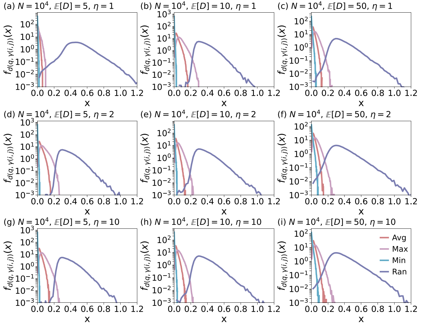
FIG. 11. The distribution of the average (avg), maximum (max), and minimum (min) distances between shortest path nodes and geodesics connecting shortest path end points in Waxman SRGGs with the connection probability function given by Eq. (4). For comparison, we also plot the distribution of distances to geodesic from randomly selected nodes (ran). The network size N = 10^4 and the parameter \beta = 1 . For each expected degree \mathbb{E}[D] and parameter \eta , we generated an SRGG and considered 10^6 random shortest paths.
