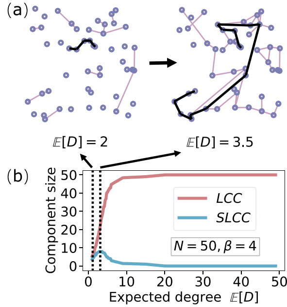
FIG. 13. (a) Visualizations of toy SRGGs with N = 50 nodes and inverse temperature \beta = 4 for increasing expected degree, from left to right: \mathbb{E}[D] = 2 , \mathbb{E}[D] = 3.5 . In each graph, a representative shortest path is highlighted in black. (b) Average sizes of the largest connected component (LCC) and the second largest connected component (SLCC) for SRGGs with N = 50 and \beta = 4 as a function of the expected degree \mathbb{E}[D] . The emergence of a giant connected component occurs at the critical expected degree D_c = 3.5 , identified by the maximum of the SLCC. All LCC and SLCC values are averaged over 100 independent realizations. Accordingly, the graph visualizations in panel (a) correspond to the disconnected and critically connected regimes.
