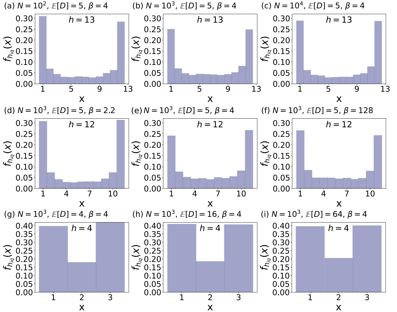
FIG. 10. Distribution of the position X of the node with the smallest distance to the geodesic along shortest paths in SRGGs for different combinations of network size N , inverse temperature \beta , and the expected degree \mathbb{E}[D] . In each panel, only shortest paths with a fixed hop count h are considered. For each shortest path, the node with the minimum distance to the geodesic is identified, and its position X \in \{1, \dots, h\} along the path is recorded. Panel (a) averages over 10^3 independent SRGG realizations, while the remaining panels correspond to a single SRGG realization. In all cases, statistics are collected from 10^5 randomly selected shortest paths per SRGG realization.
