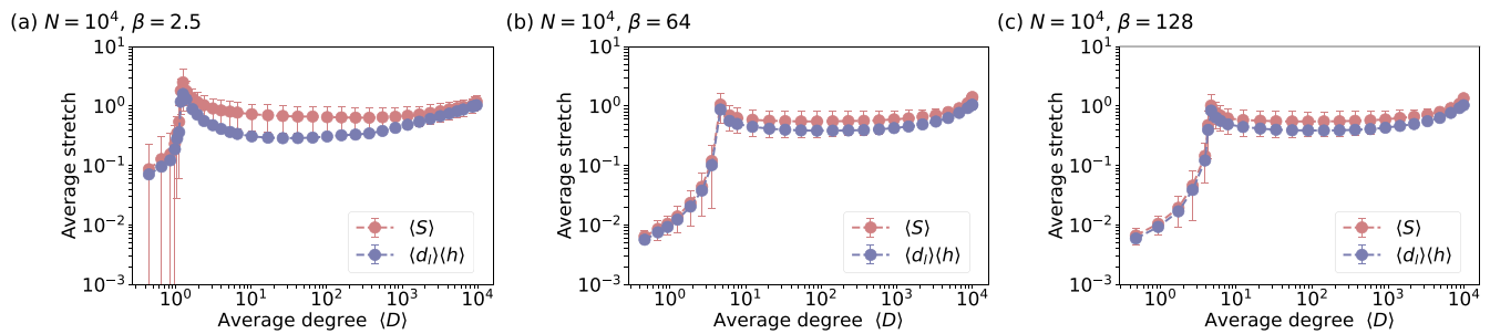
FIG. 15. Comparison of the average stretch and the product of the average link length and average hop count as functions of the average degree for SRGG networks with N = 10^4 nodes, for different values of \beta . The average stretch is computed over 10^6 randomly selected node pairs, and the error bars indicate standard deviations.
