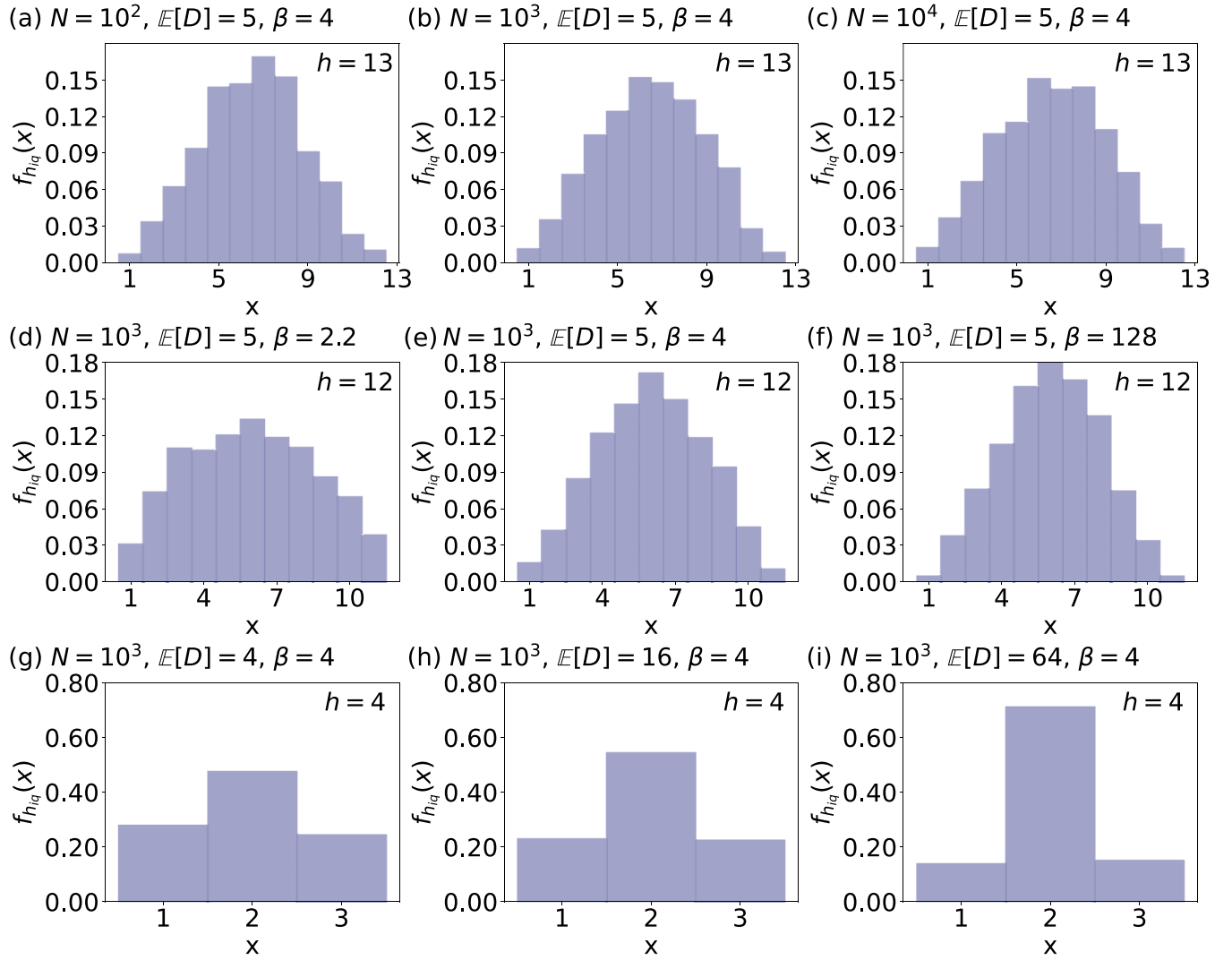
FIG. 9. Distribution of the position X of the node with the largest distance to the geodesic along shortest paths in SRGGs for different combinations of network size N , inverse temperature \beta , and the expected degree \mathbb{E}[D] . In each panel, only shortest paths with a fixed hop count h are considered. For each shortest path, the node with the maximum distance to the geodesic is identified, and its position X \in \{1, \dots, h\} along the path is recorded. Panel (a) averages over 10^3 independent SRGG realizations, while the remaining panels correspond to a single SRGG realization. In all cases, statistics are collected from 10^5 randomly selected shortest paths per SRGG realization.
