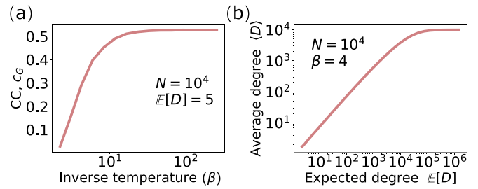
FIG. 1. Panel (a) shows an example of how the clustering coefficient changes with the input inverse temperature parameter in SRGGs. Panel (b) shows an example of how the real average degree changes with the input expected degree in SRGGs. The x axis is the input expected degree, while the y axis is the real average degree.
