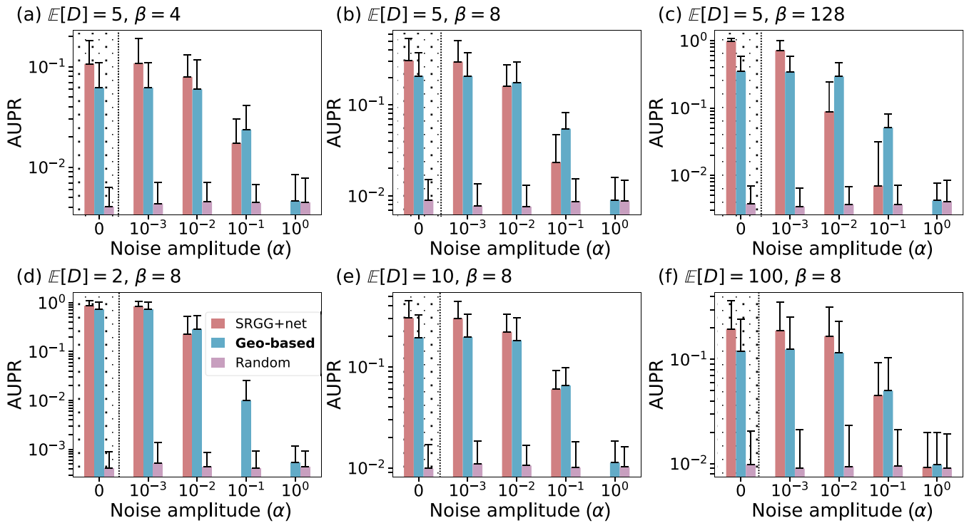
FIG. 14. AUPR of shortest path identification using the distance-to-geodesic (geometry-based) method. Panels show the average AUPR as a function of the coordinate noise amplitude \alpha , for different combinations of \mathbb{E}[D] and \beta . All experiments are performed on SRGG networks with N = 10^4 nodes. Each bar represents the average AUPR over 10^2 randomly selected node pairs and the error bars indicate standard deviations.
