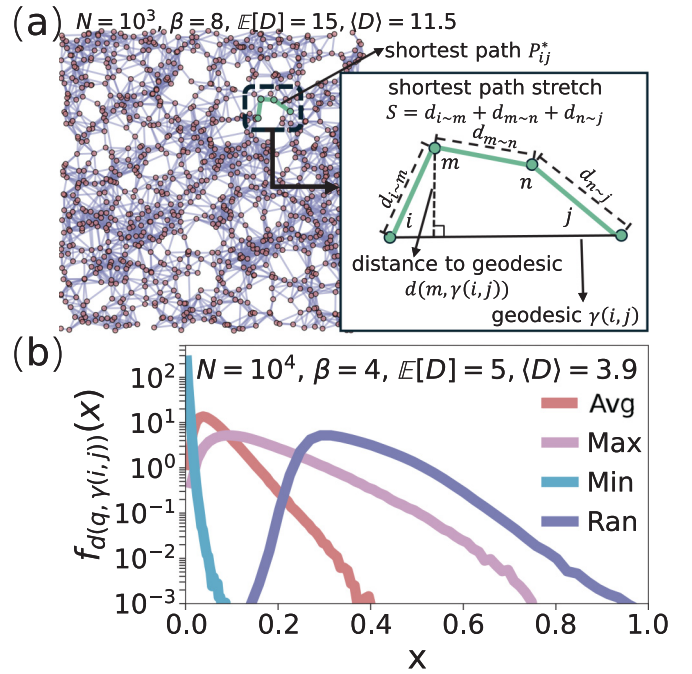
FIG. 2. (a) A toy example of a geodesic, distance from a node to the geodesic and a shortest path (highlighted by green) with the corresponding shortest path stretch indicated by the black dashed line along the green path. (b) The distribution of the average (avg), maximum (max), and minimum (min) distances between shortest path nodes and geodesics connecting shortest path end points. We compare the resulting distributions to (ran) those between randomly chosen nodes and the geodesic. Within an SRGG G , we randomly select 10^6 shortest path end point pairs and for each (i, j) pair, we find shortest path set \mathcal{P}_{ij}^* , geodesic \gamma(i, j) . For shortest path nodes in \mathcal{P}_{ij}^* , we compute the minimum (min), maximum (max), and average (avg) distance to the geodesic. In addition, for each shortest path set \mathcal{P}_{ij}^* , we created a random set \mathcal{P}_{ij}^{\text{rand}} of the same cardinality containing randomly selected nodes. Using \mathcal{P}_{ij}^{\text{rand}} , we computed average distances to the geodesic (ran). All parameters used in the experiments are indicated in the respective panels.
