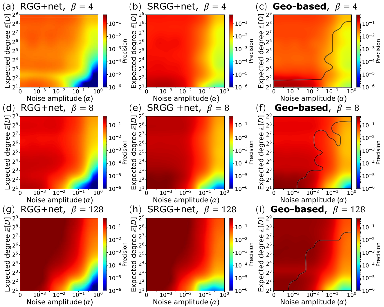
FIG. 6. Heatmap of precision. The x axis is the noise amplitude, while the y axis represents the expected degree. For each expected degree \mathbb{E}[D] and inverse temperature \beta , a 10^4 -node SRGG is generated and the coordinates are, respectively, blurred with noise amplitude \alpha . The heatmaps consist of 9 \times 9 points, each point corresponding to the average of 100 randomly selected node pairs in a (blurred) SRGG. In the region enclosed by the black line, the distance-to-geodesic approach (geo-based) achieves higher precision compared with the SRGG (SRGG+network) and RGG (RGG+network) reconstruction approaches.
