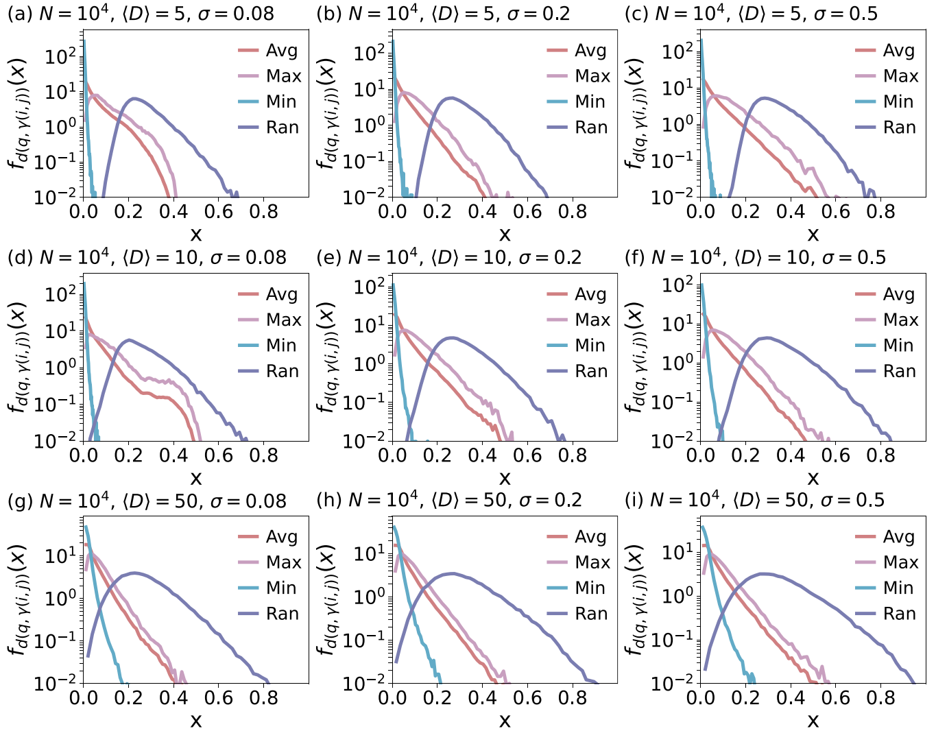
FIG. 12. The distribution of the average (avg), maximum (max), and minimum (min) distances between shortest path nodes and geodesics connecting shortest path end points in SRGGs where nodes are not uniformly scattered and the connection probability function is given by Eq. (5). The distribution of distances to geodesic from randomly selected nodes (ran) is also presented. The network size N = 10^4 . For each average degree \langle D \rangle and standard deviation \sigma of the Gaussian distribution used to sample node coordinates, we generated an SRGG and considered 10^6 random shortest paths.
