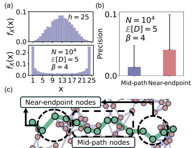
FIG. 7. [(a), top] The distribution of shortest path node positions with the largest distance to geodesic. [(a), bottom] The distribution of shortest path node positions with the smallest distance to geodesic. In both distributions, we consider shortest paths of fixed hop count, h = 25 , and SRGGs with N = 10^4 nodes, inverse temperature \beta = 4 , and the expected degree \mathbb{E}[D] = 5 . The most remote from the geodesic nodes are likely to be found in the middle of a shortest path, while the closest to the geodesic nodes are likely to be found close to the path end points. See Appendix B for plots with other SRGG parameters. (b) The precision of finding shortest path nodes near end points (near-end-point) and in the middle of the path (mid-path) using the distance to the geodesic. A 10^4 -node SRGG is generated. Each bar is the average precision computed for 100 randomly selected node pairs and the error bars depict standard deviations. Panel (c) shows an example illustrating the division of near-end-point nodes and mid-path nodes on a shortest path.
