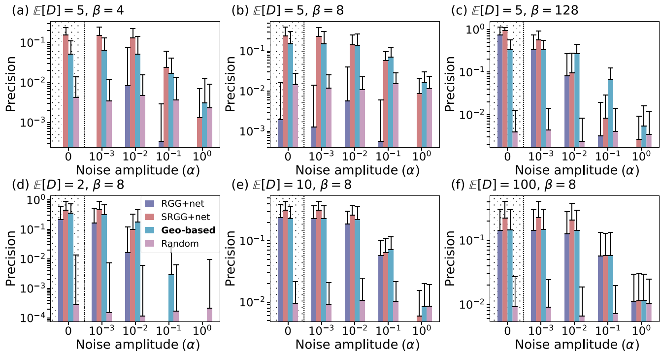
FIG. 5. Precision of shortest path finding using (1) distance to geodesic (geo-based), (2) SRGG (SRGG+network), and (3) RGG (RGG+network) reconstructions. Panels display average precision as a function of the coordinate noise amplitude \alpha and panels correspond to different combinations of \mathbb{E}[D] and \beta parameters. All experiments are performed using SRGG networks of N = 10^4 nodes. Each bar is the average precision computed for 100 randomly chosen node pairs and the error bars depict standard deviations.
