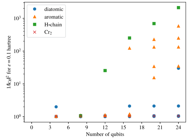
(f) 1/|c_R|^2 for energy error \epsilon = 0.1 Hartree.
