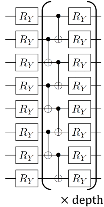
FIG. 10. Ry ansatz with eight qubits. All the rotational gates have independent parameters. The depth is set to be 8 in our experiment.
