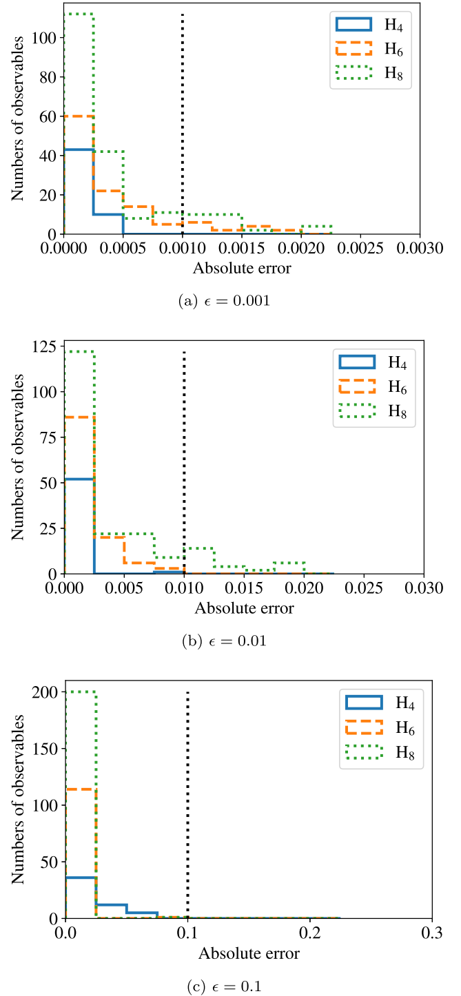
FIG. 13. Histograms of absolute errors of nuclear gradients and Hessians for \text{H}_4 , \text{H}_6 , and \text{H}_8 molecules in QSCI, compared to the exact, CASCI value. Each plot corresponds to QSCI calculations with an energy error \epsilon . Absolute errors are in units of hartree, hartree/ \text{\AA} , or hartree/ \text{\AA}^2 , depending on the observables.
