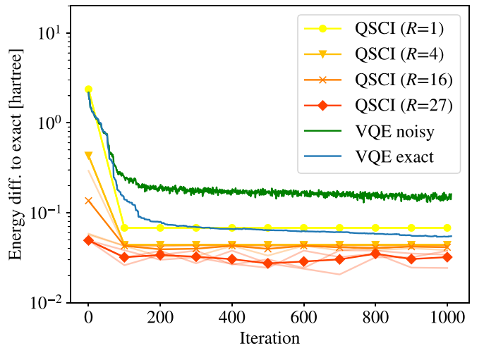
FIG. 16. Simulation results of noisy QSCI with noisy VQE input states for the hydrogen chain \text{H}_4 of eight qubits. Noisy VQE result is shown by the green line, and corresponding exact energy expectation value at each iteration is shown by the blue line. QSCI calculation is performed at every 100 iterations and the result of three trials is shown in a thin line, while the mean value is plotted in a solid line with markers.
