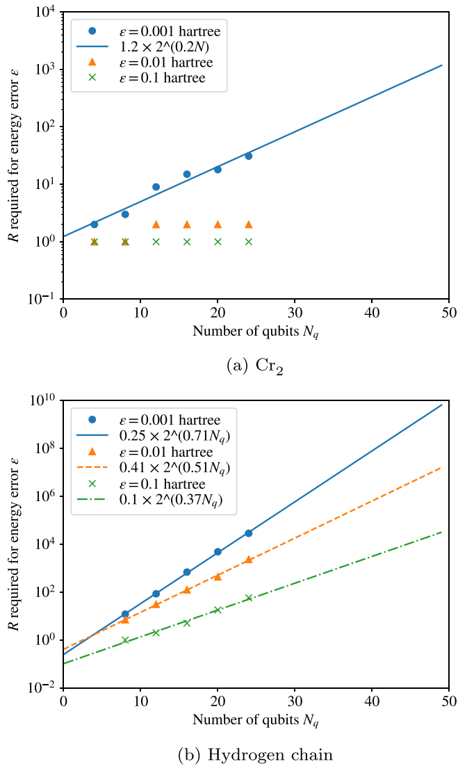
FIG. 5. Estimated R required for a given energy error \epsilon . Results with (a) expanding active spaces ( \text{Cr}_2 ) or (b) various numbers of atoms (hydrogen chain) are shown by markers, along with the linear fit of each plot.
