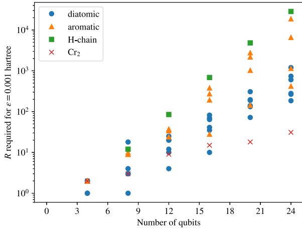
(a) R required for energy error \epsilon = 0.001 Hartree.
