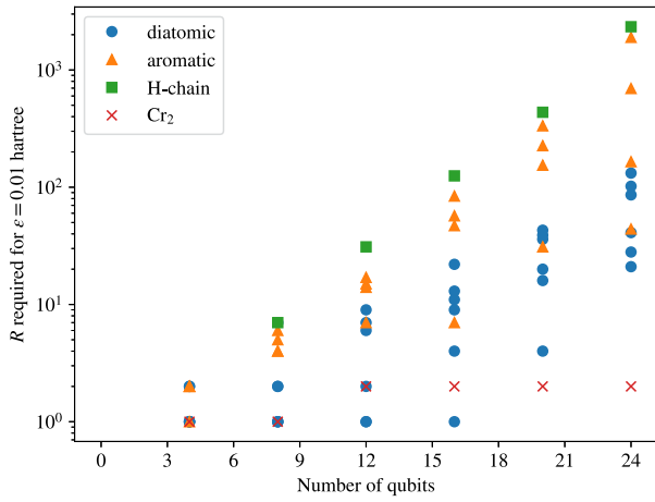
(c) R required for energy error \epsilon = 0.01 Hartree.
