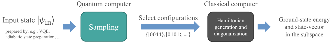
FIG. 1. Schematic description of the QSCI algorithm for finding the ground state. When selecting the configurations, one may postselect the configurations by using conserved quantities such as the electron number or spin S_z to mitigate the errors.
