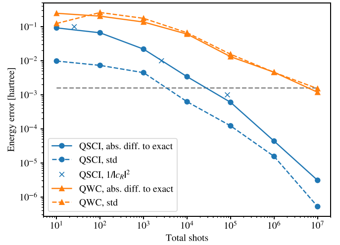
FIG. 7. Energy error results for both QSCI and conventional QWC in sampling simulations. For each set of ten trials for each method, the standard deviation and the average of the absolute error to the exact value obtained by exact diagonalization are shown. QSCI energy error using 1/|c_R|^2 shots obtained in Fig. 6 for \epsilon = 0.1, 0.01, 0.001 hartree is also plotted for reference. The horizontal line indicates the chemical accuracy, 1.6 mhartree.
