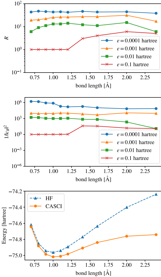
FIG. 14. Estimated R and 1/|c_R|^2 for \text{H}_2\text{O} molecule (14 qubits) with various bond lengths. Potential energy curves are also shown for reference. The estimation method of R and 1/|c_R|^2 are the same as in Figs. 5 and 6.
