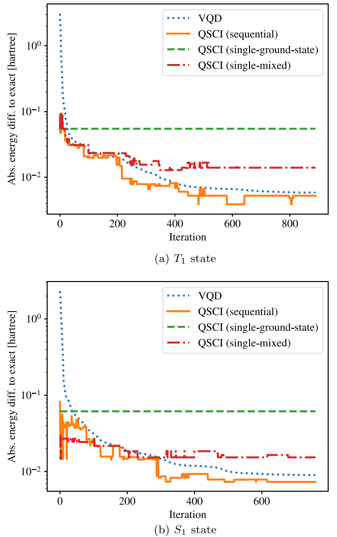
FIG. 4. Same as Fig. 3 but for (a) ( T_1 ) and (b) ( S_1 ) excited states of \text{H}_2\text{O} with S_z = 0 , along with optimization histories of VQD, shown by dotted lines, for input-state preparation; the energy differences are plotted by the absolute values. For the QSCI calculation of the T_1 ( S_1 ) state, the input state(s) corresponding to the lower energy states, i.e., S_0 ( S_0 and T_1 ) state(s), are prepared by converged sets of parameters of VQD. QSCI results are shown for the sequential diagonalization and the single diagonalization with two types of configuration selection, as described in the main text. The QSCI calculations with sequential diagonalization are done with R_i = 16 for i = 0, 1, 2 , while the value of R is set to R = 16 for single diagonalization.
