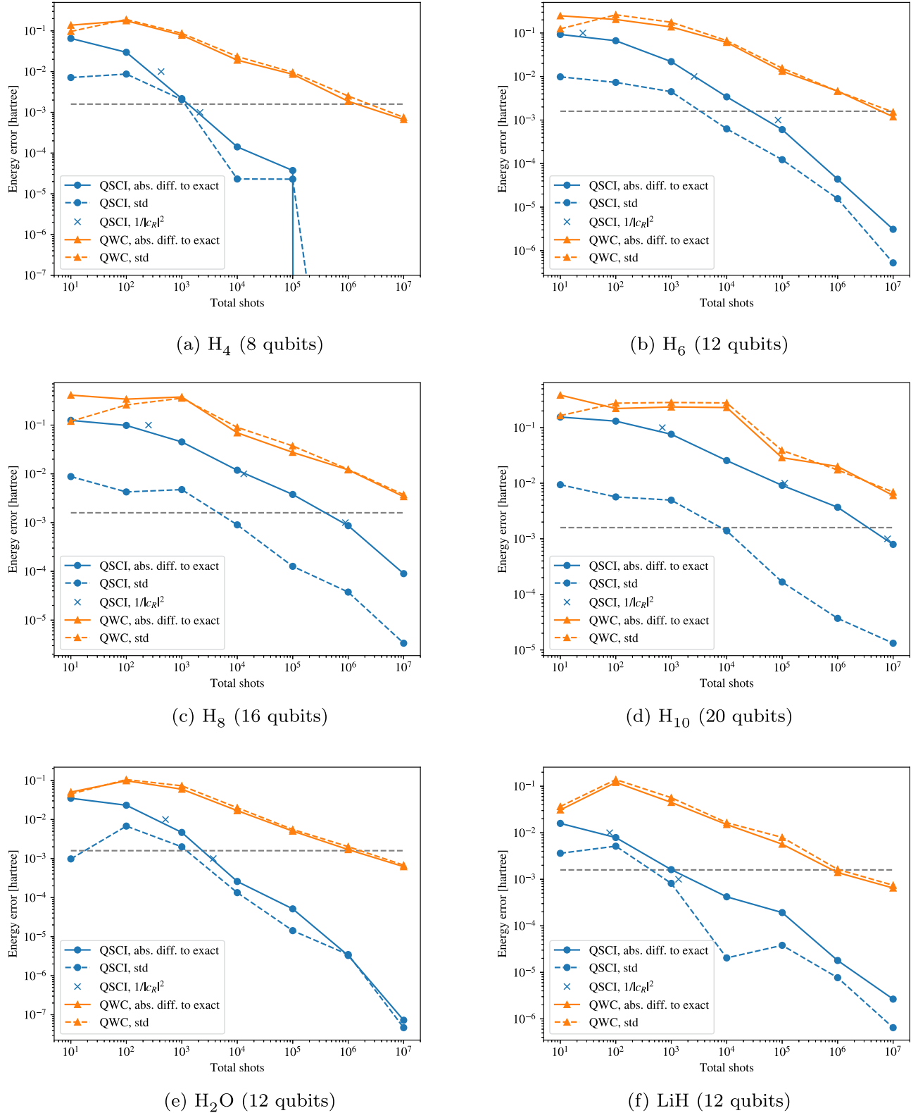
FIG. 12. Sampling simulation with various molecules. See Fig. 7 and the main text for details.
