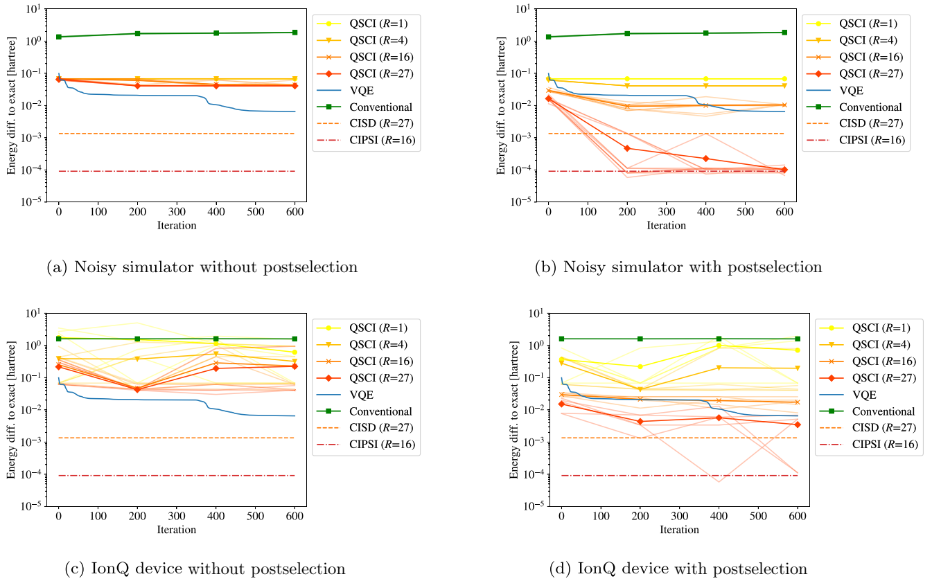
FIG. 8. QSCI results for the ground state of the linear hydrogen chain H_4 with eight qubits by the noisy simulator [panels (a) and (b)] and by the IonQ device [panels (c) and (d)], with and without postselection, compared with the conventional method of quantum-expectation-value estimation and classical computational methods. The resulting energies are plotted in hartree as deviations from the one obtained by the exact diagonalization (CASCI). The conventional method uses the QWC grouping in the energy estimation. Two classical methods are plotted for reference: CISD uses 27 Slater determinants, and we chose 16 Slater determinants for CIPSI, which is sufficient to achieve 0.1 mhartree accuracy. Lines specified by “VQE” show the exact energy value of the parametrized state at each iteration, and the states at four selected iterations are used as the input states for the QSCI calculations, shown by “QSCI” with four different values of R . The markers on the solid lines show the average value of some trials while each line without markers shows the result of each trial. The number of trials is ten for both QSCI and the conventional method on the noisy simulator, one for the conventional method, and five for QSCI, both on the IonQ device.
