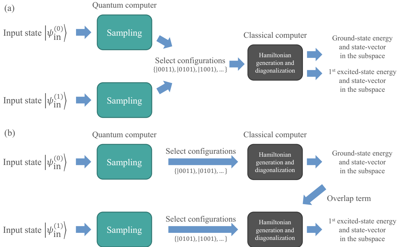
FIG. 2. Schematic descriptions of the QSCI algorithms for finding the ground state and the first excited state: (a) single diagonalization scheme and (b) sequential diagonalization scheme. In both panels, |\psi_{\text{in}}^{(0)}\rangle ( |\psi_{\text{in}}^{(1)}\rangle ) is the input state for the ground (first excited) state. In panel (b), the overlap term is constructed from the preobtained output state |\psi_{\text{out}}^{(0)}\rangle to define the effective Hamiltonian for the first excited state, \hat{H}^{(1)} = \hat{H} + \beta_0 |\psi_{\text{out}}^{(0)}\rangle \langle \psi_{\text{out}}^{(0)}| .
