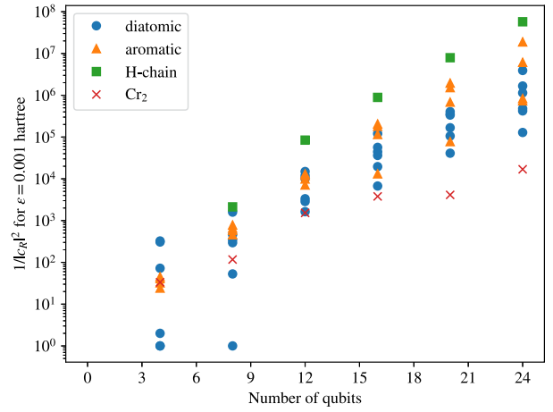
(b) 1/|c_R|^2 for energy error \epsilon = 0.001 Hartree.
