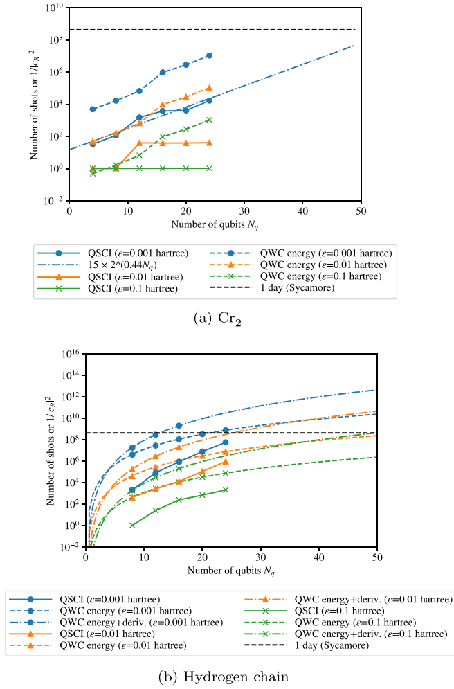
FIG. 6. Estimated number of shots for a given energy error \epsilon . For QSCI, the number of shots is approximated by 1/|c_R|^2 , where R for each \epsilon is obtained in Fig. 5 and c_R is the CI coefficient of the input state with R th largest absolute value. The reasoning for this approximation is explained in the main text. For comparison, the results of the conventional expectation-value estimation with QWC grouping are plotted for each \epsilon , fitted by a logarithmic function in the plot: The required numbers of shots for evaluating the energy are shown by dashed curves; for hydrogen chains, the ones for evaluating the gradients and Hessians in addition to the energy are shown by dash-dotted curves; the precision of gradients and Hessians are set to be \epsilon/\text{\AA} and \epsilon/\text{\AA}^2 , respectively. The number of shots that can be executed on Google's Sycamore processor [1], which can perform a million shots in about 200 s, is plotted in black dashed line. For panel (a), we also plot a linear fit of the QSCI results with \epsilon = 0.001 hartree, for reference.
