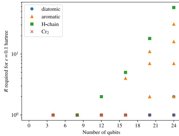
(e) R required for energy error \epsilon = 0.1 Hartree.
