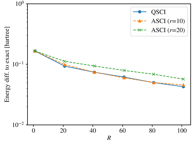
FIG. 15. Comparison of ASCI and QSCI for \text{H}_{10} molecule (20 qubits). The ASCI and QSCI energies as the difference to the exact CASCI energy are plotted against the size R of the selected subspace. The parameter r determines the size of the search space for ASCI.
