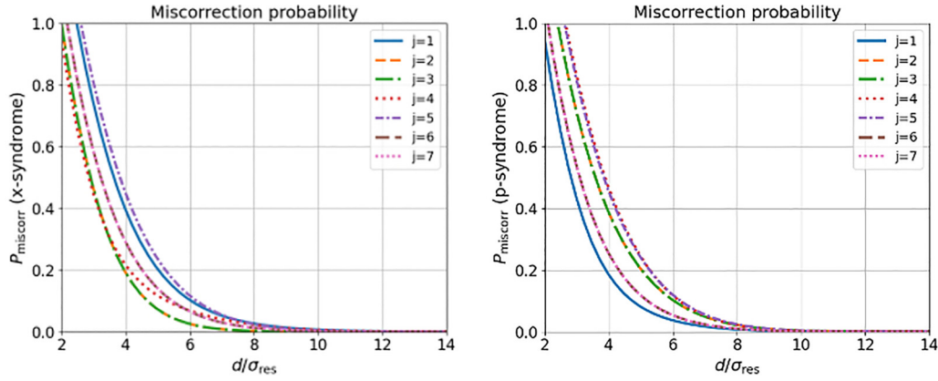
FIG. 6. Mis-correction probability P_{\text{miscorr}}^{(j)} as a function of the normalized ratio d/\sigma_{\text{res}} . The index j = 1, \dots, 7 labels the qumode position within the seven-mode analog Steane encoding block (ordered from top to bottom in the encoding circuit). A mis-correction event refers to the situation in which a displacement error occurring on the j th qumode is incorrectly localized due to residual Gaussian displacement noise. In the calculation, a displacement error of magnitude d is applied to a given qumode j , while each mode carries residual Gaussian displacement noise with standard deviation \sigma_{\text{res}} . The analog Steane code attempts to identify the error location using its syndrome information. Gaussian errors may distort the inferred syndrome values, leading to a nonzero probability of incorrect localization. Each curve shows this probability for a given j . The left panel corresponds to the position quadrature ( x ) and the right panel corresponds to the momentum quadrature ( p ). The mis-correction probability decreases as d/\sigma_{\text{res}} increases, since larger displacement magnitudes are less affected by the same level of residual Gaussian noise [44].
