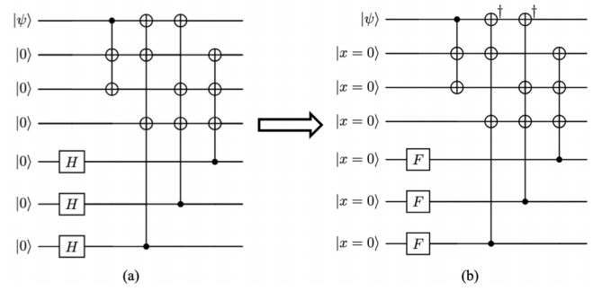
FIG. 1. (a) DV Steane code. (b) Analog Steane code obtained by replacing the H and cnot gates with F and sum (or \text{SUM}^\dagger ) gates.
