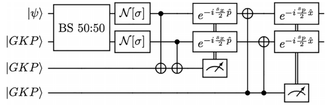
FIG. 4. Gaussian-error-suppression circuit.
