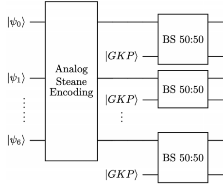
FIG. 5. Schematic diagram of the concatenated circuit combining the analog Steane encoding and the Gaussian-error-suppression circuit.
