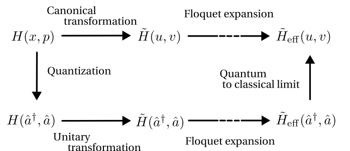
FIG. 6. Diagram highlighting the correspondence between the classical Krylov-Bogoliubov and quantum Van Vleck Floquet expansions to obtain an effective Hamiltonian for the stroboscopic dynamics.
