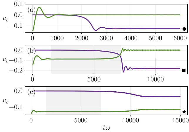
FIG. 4. Temporal evolution of the quadrature u of the S and A modes, starting from the same antisymmetric initial condition. (a) Outside the parametric interaction region (cf. circle marker in Fig. 2), the antisymmetric state |\uparrow\downarrow\rangle_{\mathcal{N}} quickly decays while the symmetric mode rings up to a finite amplitude. (b) Inside the parametric interaction region \Pi_a (cf. square marker in Fig. 2), the antisymmetric state persists (gray region) before decaying due to the parametric amplification of the symmetric mode. (c) Inside the parametric interaction region \Pi_b (cf. star marker in Fig. 2), the antisymmetric state persists (gray region) while ringing up the symmetric mode, yielding a mixed-symmetry stationary state.
