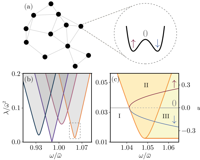
FIG. 1. Characterization of a KPO network [cf. Eq. (1)]. (a) Sketch of a coupled KPO network, where the motion of each mode is effectively described via a rotating quasienergy potential, which has up to three possible stable states. The latter form an effective spin-1 subspace \{\uparrow, \downarrow, 0\} (see Sec. II C). (b) The stability diagram around the first instability lobe for different linear parametric resonators, e.g., modes of a decoupled KPO network, or linear normal mode of the coupled system, as a function of the dimensionless parametric pump amplitude \lambda/\bar{\omega}^2 and driving frequency \omega/\bar{\omega} (see Sec. II A). The frequency \bar{\omega} is chosen to be the mean of the natural frequencies of the individual lobes. The gray regions indicate where the k th linear mode becomes parametrically unstable. (c) The I (white), II (orange), and III (yellow) regions denote parameter regimes where only the zero-amplitude state, only the phase state, or both zero-amplitude and phase states are stable, respectively (see Sec. II B). The quadrature u_k of the stationary-state solutions as a function of \omega for a cut at \lambda = 0.03 is superimposed onto the phase diagram.
