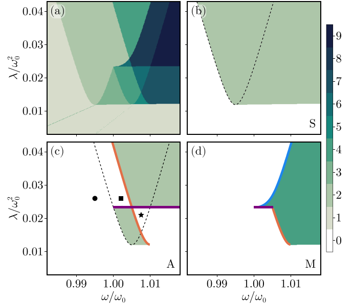
FIG. 2. Phase diagram of two homogeneously coupled KPOs with bare frequencies \omega_0 [cf. Eqs. (11) and (12) and Appendix C], as solved by HarmonicBalance.jl [42]. (a) Number of stable states as a function of the dimensionless parametric pump amplitude \lambda/\omega_0^2 and driving frequency \omega/\omega_0 , with \gamma/\omega_0 = 0.006 and J/\omega_0^2 = 0.01 . The states can be classified into (b) symmetric, (c) antisymmetric, and (d) mixed-symmetry states, yielding their own respective stability phase diagrams. Dashed lines mark the Arnold tongue of the symmetric and antisymmetric mode in the absence of cross-Kerr terms in panels (b) and (c), respectively. Solid colored lines mark the modified parametric instability lines due to cross-Kerr coupling [cf. Eqs. (13) and (14)]. Black square and circle mark the parameters used in Fig. 4.
