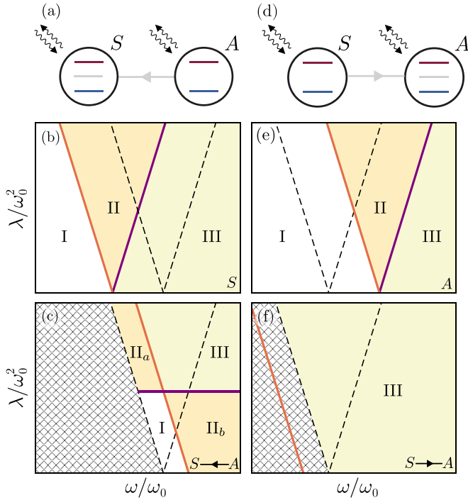
FIG. 3. Influence of the cross-nonlinearity coupling between the S and A normal modes of two homogeneously coupled KPOs with J > 0 and \alpha > 0 [cf. Eqs. (11) and (12)]. (a) and (d) Illustration of the directional perturbative schemes of how the A (S) mode (circles with lines marking spin-1 states) parametrically drives (directional arrow) the S (A) mode [cf. Eqs. (13)]. (b) and (e) Phase diagram of the uncoupled S (A) mode. The I (white), II (orange), and III (yellow) regions denote the regions where only the zero-amplitude state, only the phase state, or both zero-amplitude and phase states are stable, for the given normal mode, respectively. The black dashed lines indicate the parametric lobe (bifurcation lines) of the other mode. (c) and (f) State-dependent stability diagram for the S (A) mode perturbed by an A (S) oscillation [cf. Eq. (13)]. Inside the dashed region, the A (S) mode can only have a zero amplitude; hence, no state-dependent stationary states of S (A) exist. The orange and purple lines indicate the state-dependent bifurcation lines of the S and A modes, respectively [cf. Eqs. (14) and (15)].
