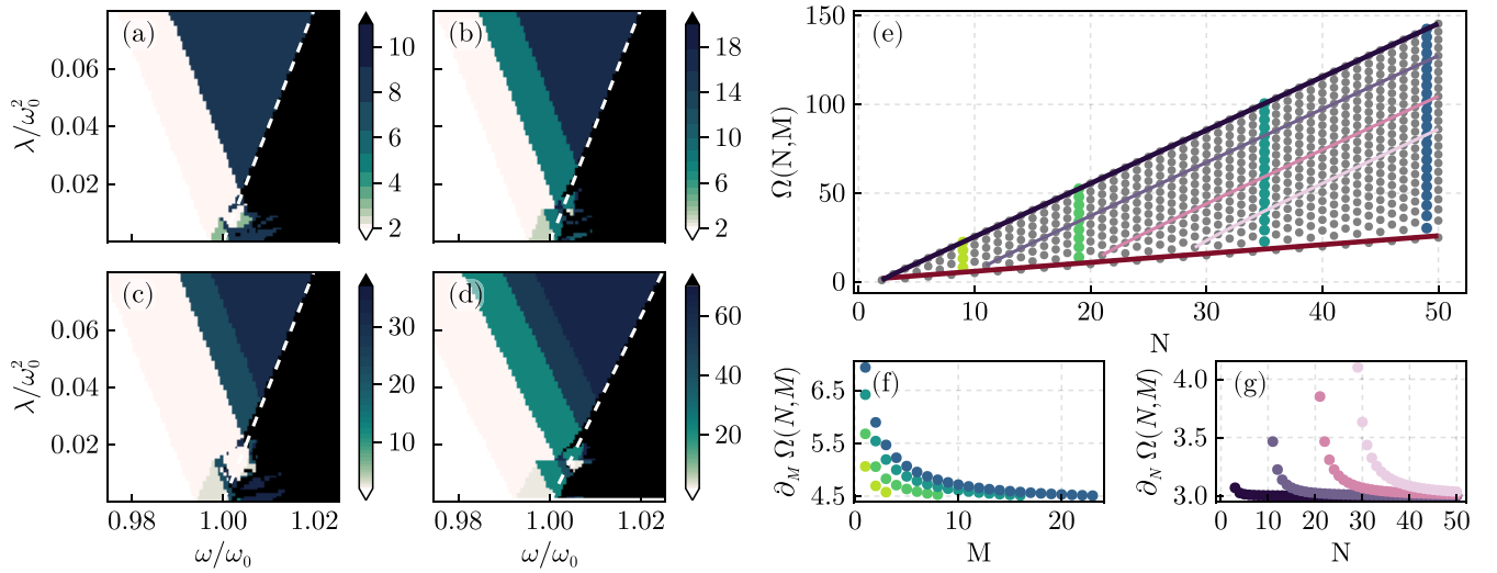
FIG. 5. Stability phase diagrams and frequency shifts for homogeneously coupled KPO networks. (a)–(d) Stability phase diagrams for networks of three to six coupled KPOs, respectively, as solved by HarmonicBalance.jl [42]. It shows the number of stable states as a function of the dimensionless parametric pump amplitude \lambda/\omega_0^2 and driving frequency \omega/\omega_0 , with \gamma/\omega_0 = 0 and J/\omega_0^2 = 0.003 . The color scale is capped at 2^N to highlight the regions where the number of stable states matches the number of Ising states in a network with N nodes. The white dashed lines represent the bifurcation line \lambda_+^{(1/2)}(\omega) from Eq. (16). Note that while panels (b) and (c) have the same number of bifurcation lines, the number of stable states differs, as indicated by the color bar. White regions appearing for small \lambda correspond to instabilities in the model that disappear when finite damping is added. They are not further investigated in this work, as they are not observable in experiments. (e) Frequency shift \Omega(N, M) [cf. Eq. (22); gray dots] for every partition \{n = (1/2)(N + M), m = (1/2)(N - M)\} up to N = 50 . The trend lines for partitions \{N - 9, 9\} , \{N - 19, 19\} , and \{N - 27, 27\} are indicated in increasingly lighter shades of purple. (f) Difference in frequency shift \Omega(N, M) with respect to M for network sizes N = 9, 19, 35, 49 , showing a convergence to 9/2 [cf. Eq. (23)]. (g) Difference in frequency shift \Omega(N, M) with respect to N , indicating a uniform spacing between bifurcation lines in the large- N limit [cf. Eq. (24)].
