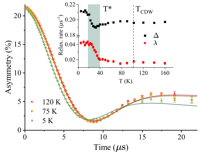
FIG. 1. The ZF- \mu SR spectra of \text{RbV}_3\text{Sb}_5 . The main panel depicts three high-statistics acquisitions showing the evolution of the asymmetry as a function of the temperature. A tiny difference is observed between signals above (120 K) and below (75 K) the CDW transition (102 K). A noticeably faster relaxation is instead observed in the measurement performed at 5 K. The continuous lines are best fits to Eq. (1). The inset shows the temperature evolution of the fitting parameters resulting from the analysis described in the main text.
