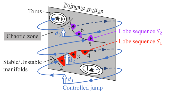
FIG. 2. Schematic view of our control. The start point, goal point, and centers of gravity of the lobes are denoted as a triangle, a star, and black dots, respectively. Finitely long effective lobe sequences S_i ( i = 1, 2 ) are used for the transfer. In this example, three controlled jumps outside the Poincaré section are required to connect two orbits in different elliptic islands. The numbers indicate the order of the transfer. The total control cost D = \sum_{k=1}^N d_k ( N = 3 here) is minimized.
