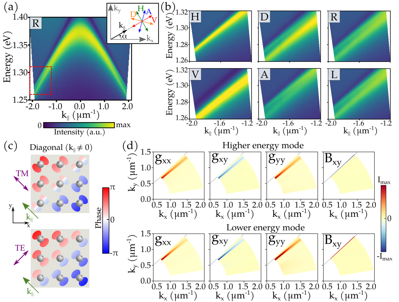
FIG. 2. (a) Transmission measurements at the diagonal of the Brillouin zone ( \alpha = 45^\circ ) for right (R) circular polarization. (b) Measurements in the red-dashed square of (a) with horizontal (H), vertical (V), diagonal (D), antidiagonal (A), right, and left (L) circular polarization filtering. (c) Explanation of TE-TM band splitting along one diagonal of the first Brillouin zone (with k_{||} \neq 0 ). The same phase distribution is created in real space for both TE and TM polarizations, but unlike in Fig. 1(a), the radiation patterns are only approximately TE or TM due to the non-Hermiticity, but we name them TE and TM for practical reasons. (d) Quantum metric and Berry curvature for the higher and lower energy modes in (a) and (b), for 10^\circ < \alpha < 45^\circ . The magnitude I_{\text{max}} of the Berry curvature is 10^{-3} times smaller than the quantum metric components. The grey-dashed line marks the diagonal of the Brillouin zone.
