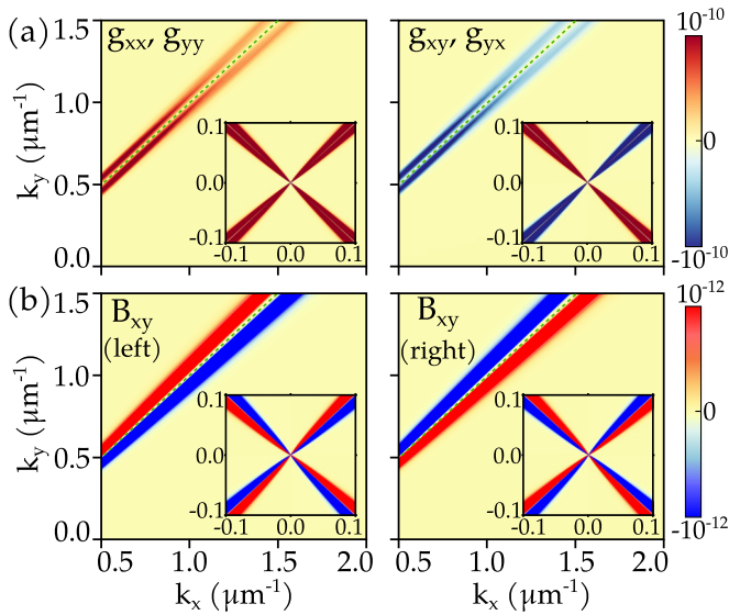
FIG. 3. QGT obtained with the two-band model. Main panels show the same area of the Brillouin zone as the experiments in Fig. 2(d), and the insets display neighboring regions to the \Gamma point. The green dashed line marks the diagonal of the Brillouin zone. (a) Quantum metric components. We find that g_{xx} = g_{yy} = -g_{xy} = g_{yx} . (b) Berry curvature calculated with the right and left eigenvectors of the Hamiltonian. We found that \mathfrak{B}_{xy}^n = -\mathfrak{B}_{yx}^n . Colorscale units are \text{m}^2 .
