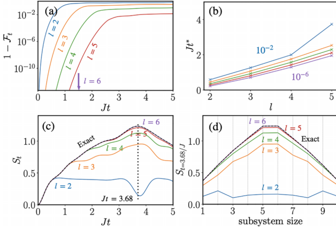
FIG. 3. The infidelity and von Neumann entropy in the global quench dynamics for the L = 11 quantum Ising chain with the model parameters g = 1.4 and h = 0.1 in the nonintegrable region. The time-evolved state |\Psi(t)\rangle is approximated using the single-layer sequential-type quantum circuits consisting of l -qubit gates, |\Phi(t)\rangle = \hat{C}_l|\Phi\rangle (see Fig. 2). (a) Time evolution of the infidelity 1 - \mathcal{F}_t for different gate sizes. The arrow indicates the infidelity 1 - \mathcal{F}_t lower than 10^{-14} . (b) The maximum evolution time t^* below which 1 - \mathcal{F}_t < 10^{-z} ( z = 2, 3, \dots, 6 ) as a function of the gate size l . (c) Time evolution of the von Neumann entropy S_t for different gate sizes. Here, the system is partitioned into subsystems of five and six sites. The vertical dotted line highlights the evolution time at which the numerically exact time-evolved state |\Psi(t)\rangle exhibits the maximal von Neumann entropy, i.e., Jt = 3.68 . (d) The subsystem size dependence of the von Neumann entropy S_t evaluated at Jt = 3.68 . For comparison, the numerically exact results evaluated from |\Psi(t)\rangle are also plotted by the dashed lines in (c) and (d). The hyperparameters are set to be w_{\max} = 10^4 , w_{\min} = 10^2 , \epsilon_a = 10^{-14} , and \epsilon_r = 10^{-4} .
