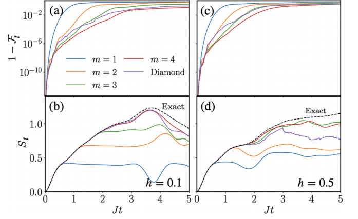
FIG. 7. Time evolution of [(a), (c)] the infidelity 1 - \mathcal{F}_t and [(b), (d)] the von Neumann entropy S_t for the m -layer sequential-type quantum circuits consisting of two-qubit gates and the diamond-shaped quantum circuit in the case of a finite longitudinal magnetic field [(a), (b)] h = 0.1 and [(c), (d)] 0.5 . Other model parameters and the hyperparameters for the circuit optimization are the same as those in Figs. 6(a) and 6(b).
