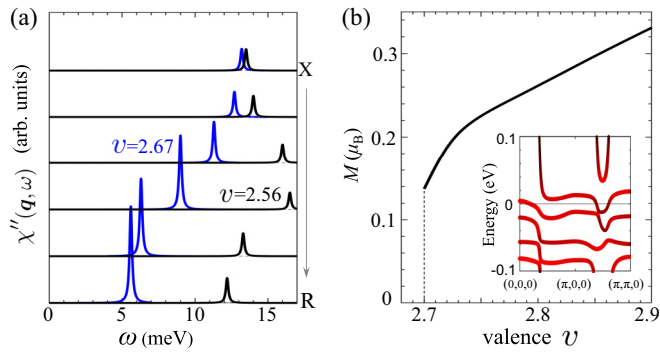
FIG. 2. (a) Dynamical magnetic susceptibility \chi''(\mathbf{q}, \omega) for the valence v = 2.56 (black) and 2.67 (blue), for \mathbf{q} values along the high symmetry path from X = (\pi, 0, 0) to R = (\pi, \pi, \pi) . The particle-hole continuum (not shown) is above \simeq 17 meV. (b) The G-type ordered magnetic moment M as a function of v . The inset shows the metallic band structure at v = 2.72 .
