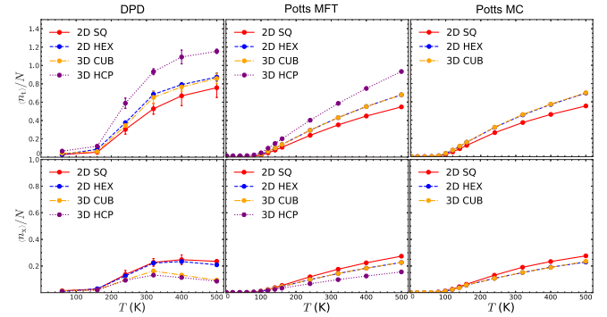
FIG. 3. Comparison of links across 2D SQ, 2D HEX, 3D CUB, and 3D HCP arrays. The first, second, and third columns correspond to DPD, Potts model MFT, and Potts model MC, respectively. The first row reports the total numbers of links. The second row reports the average number of links in the x direction. The normalization factor N = 100, 100, 125 , and 180 in 2D SQ, 2D HEX, 3D CUB, and 3D HCP, respectively. The other links and sum of nearest-neighbor links from DPD simulations are available in Fig. S7 in SM [37].
