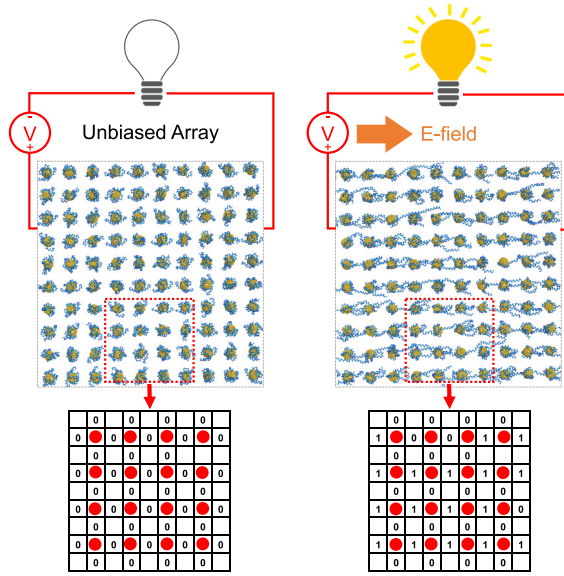
FIG. 1. Scheme of an electric-field-induced network structure changing in 2D SQ regular arrays. The detailed simulation model is described in Ref. [29] and Fig. S1 in SM [37].
