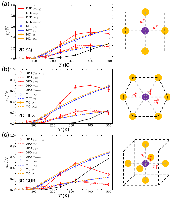
FIG. 2. Comparisons of network connections in (a) 2D SQ, (b) 2D HEX, and (c) 3D CUB at T ranging from 30 to 500 K under no E field. Observations of DPD simulations are compared to the Potts model from MFT and MC. Diamond symbols represent the sum of nearest-neighbor links. Small dots represent nearest-neighbor links in each direction. Black solid lines represent other types of links. The normalization factor N is the total number of ENPs in the array; here, N = 100 in both 2D SQ and 2D HEX, N = 125 in 3D CUB.
