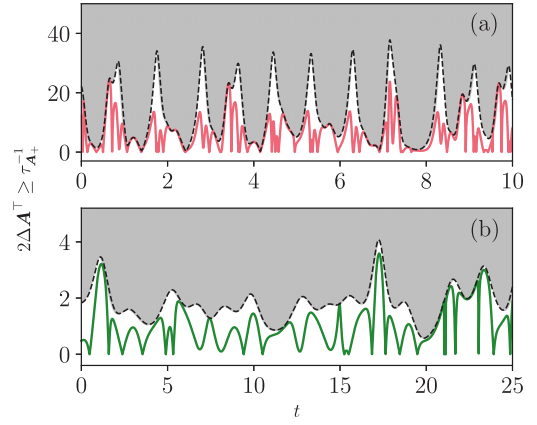
FIG. 2. Speed limit on chaos. The instantaneous Lyapunov exponent, r(t) = \langle \mathbf{A}_+ \rangle , for phase-space orbits of (a) the Lorenz-Fetter model and (b) the Hénon-Heiles model. Square root of the tangent-space Fisher information (dashed black) \sqrt{\mathcal{I}_F} = 2 \Delta \mathbf{A}^T upper bounds the speed \tau_{\mathbf{A}_+}^{-1} (solid red and green). Shaded regions mark speeds not accessible to the observable. The parameters of the Lorenz-Fetter model are: \sigma = 10 , \beta = 8/3 , and \eta = 22 (transient chaos). For the Hénon-Heiles system, the chaotic trajectory corresponds to the energy E = 1/6 .
