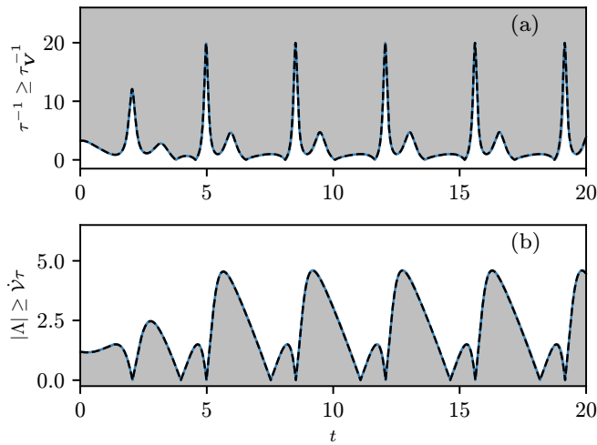
FIG. 1. Speed limit on the dissipation rate of the van der Pol oscillator. (a) The Fisher information \tau^{-1} = \sqrt{\mathcal{I}_F} = 2 \Delta \mathbf{A}^\top upper bounds (dashed black curve) the intrinsic speed \tau_V^{-1} of dissipation \Lambda = \langle \mathbf{V} \rangle with respect to a normalized perturbation \mathbf{q} (solid blue): \tau^{-1} \geq \tau_V^{-1} . (b) The inequality also sets a lower bound on the magnitude of dissipation |\Lambda| \geq \dot{\mathbf{V}}\tau . Panel (b) shows |\Lambda| (solid blue curve) is bounded from below by \dot{\mathbf{V}}\tau (dashed black curve). The trajectory is on the stable limit cycle with damping parameter \mu = 1.5 . Shaded regions mark regimes inaccessible to \tau_V^{-1} and |\Lambda| .
