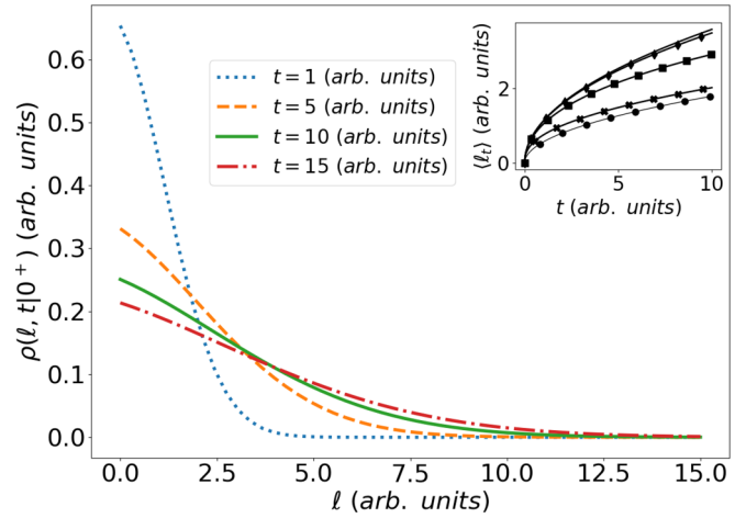
FIG. 3. The barrier local time distribution for \kappa = 0.1 and D = 1 (in arbitrary units), computed via a numerical inverse Laplace transform [38] of Eq. (17) and plotted against \ell at different times t = 1, 5, 10, 15 , respectively. The inset: the mean barrier local time Eq. (18) plotted over a time window for varying permeability values \kappa = \infty, 1, 0.1, 0.01, 0 (in arbitrary units) represented by the markers: circular, cross, square, diamond, and no marker, respectively. For \kappa \rightarrow \infty , we have the barrier free mean local time \sqrt{t/\pi D} and for \kappa \rightarrow 0 , we have the perfectly reflecting barrier mean local time 2\sqrt{t/\pi D} .
