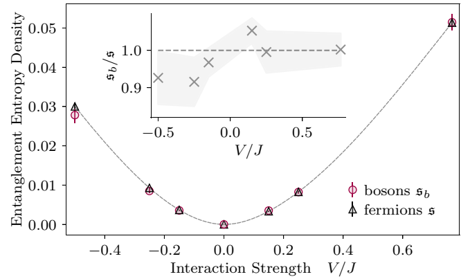
FIG. 4. Entanglement entropy density. We compare the steady-state spatial entanglement entropy density \mathfrak{s} for fermions with the entropy density \mathfrak{s}_b computed from a bosonic diagonal ensemble of density excitations Eq. (6). The bosonic occupation numbers \langle n_q \rangle were obtained from an analysis of the data presented in Fig. 2. The dashed line is a guide to the eye. The ratio of the two entropy densities is consistent within error bars (inset).
