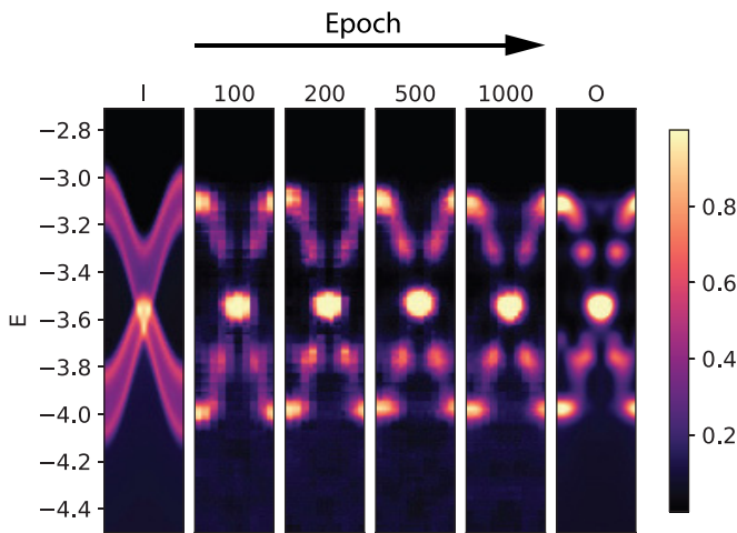
FIG. 7. Evolution of the CNN prediction quality with increasing training time on an Hamiltonian sampled from M10. Input (I) is the LDOS calculated from the aligned bilayer Hamiltonian and output (O) is the LDOS calculated from the moiré bilayer Hamiltonian. The panels in the middle show the predicted LDOS from neural network after corresponding 100, 200, 500, and 1000 epochs.
