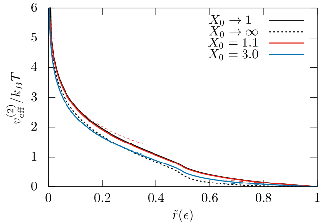
FIG. 3. Numerical results for v_{\text{eff}}^{(2)}(r) and X_0 = 1.1 (solid red line) and 3.0 (solid blue line) for a 2D fluid of ellipses with semiaxes of length a, b and aspect ratio X_0 = a/b = 1 + \epsilon as a function of the scaled distance \tilde{r}(\epsilon) = (r/2b - 1)/\epsilon . Also shown are the semi-analytical results, Eqs. (A10) and (A11), for X_0 \rightarrow 1 (upper black solid line) and Eqs. (A21)–(A23) for X_0 \rightarrow \infty (lower black dotted line) as well as the analytical asymptotic results, Eqs. (A16) and (A15), for r \rightarrow 2b^+ and r \rightarrow 2a^- , respectively (corresponding to dashed lines).
