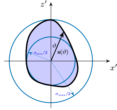
FIG. 1. Construction for an arbitrary 2D convex hard body, B , (blue domain) of the smaller ( S_{\min} ) and larger circle ( S_{\max} ) with radius \sigma_{\min}/2 and \sigma_{\max}/2 , respectively. The center of B is chosen as the origin of the body-fixed frame and the z' axis points to the tangential contact of B and S_{\max} . The shape of the hard body is parametrized by \mathbf{s}(\vartheta) where \vartheta is the angle between \mathbf{s}(\vartheta) and the z' axis (see also main text).
