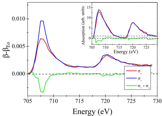
FIG. 3. The complex part of the refractive index vs energy obtained from the fitting of the interferogram. Inset showcases the diode current values normalized as a measure of XMCD absorption. The red, blue, and green curves correspond to \sigma_- light, \sigma_+ light, and the dichroic signal ( \sigma_+ - \sigma_- ), respectively.
