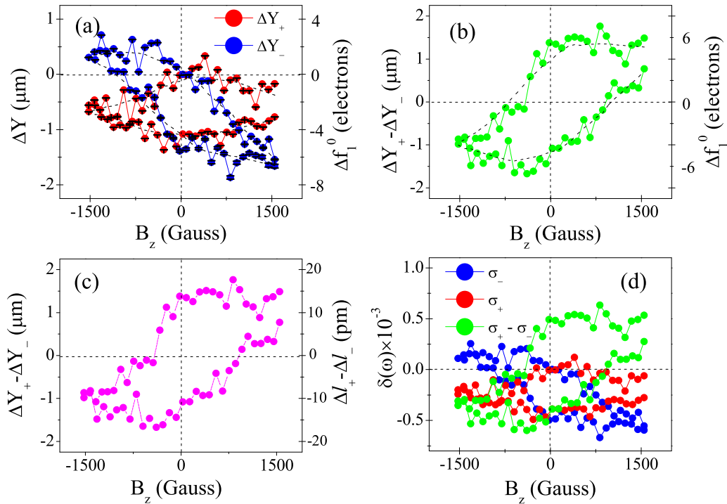
FIG. 2. Experimental fringe shift recorded through the magnetic hysteresis. Panel (a) shows the registered fringe displacement for circularly polarized light. The error bars are smaller than the data points (visible upon magnifying the image). Data in the subsequent panels are derived from panel (a). Error bars are not displayed. Panel (b) shows the difference between the two curves. The axis on the right-hand side shows the corresponding change in the scattering factor values ( \Delta f_1^0 ). Panel (c) shows the difference between the two curves scaled to the difference in the magnetic path length. Panel (d) shows the hysteresis curves for \sigma_+ , \sigma_- , and \sigma_+ - \sigma_- light scaled to display the changes in their respective \delta(\omega) values with respect to their \delta values at B_z = 0 G.
