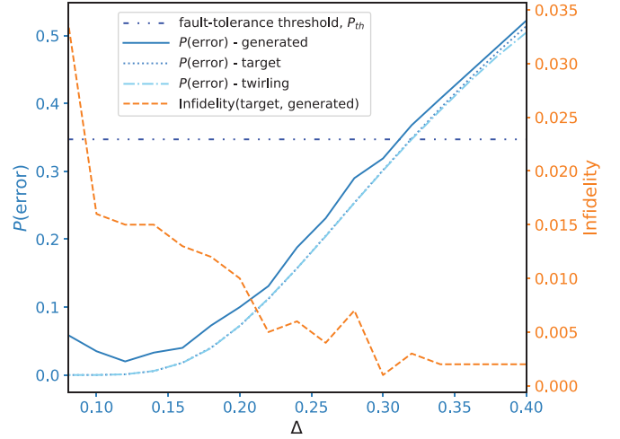
FIG. 3. Error probability, calculated using Eq. (A1), for target GKP |\tilde{0}\rangle and generated states with different values of \Delta , the inverse width. We show the error probability for the twirling states used in Ref. [90], as well as the fault-tolerance threshold. The infidelity between the target and generated GKP states is also plotted.
