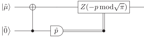
FIG. 4. Quantum circuit for correcting momentum errors in an approximate GKP state, |\tilde{\mu}\rangle , using an auxiliary GKP qubit, |\tilde{0}\rangle [51,91]. An inverse-SUM gate, \exp[i\hat{q}_1\hat{p}_2] , acts on the inputs. Then, the second mode is measured in the momentum basis and the measurement outcome, p , is fed to a displacement gate, Z(-p \bmod \sqrt{\pi}) . Notice that all the elements of the circuit are comprised in our LB universal model.
