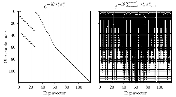
FIG. 11. Sparsity of gates generated by Pauli strings versus general gates. We plot sparsity maps for the eigenvector matrix \bar{\mathbf{Q}} where \Phi_\lambda^{\text{Ad}} \exp(-i\theta H) = \bar{\mathbf{Q}} \text{diag}(e^{-i\theta \epsilon^{(1)}}, \dots, e^{-i\theta \epsilon^{(\dim(\mathcal{L}_\lambda))}}) \bar{\mathbf{Q}}^T , for H = \sigma_1^x \sigma_2^x (left) and H = \sum_{m=1}^{n-1} \sigma_m^x \sigma_{m+1}^x (right), for a system of n = 8 qubits in the \mathcal{L}_\lambda = ig_0 representation. White (black) entries in the map indicate (nonzero) zero entries. The gate \exp(-i\theta \sigma_1^x \sigma_2^x) has a sparse eigenvector matrix since it is generated by a single Pauli string, whereas the gate \exp(-i\theta \sum_{m=1}^{n-1} \sigma_m^x \sigma_{m+1}^x) has a dense eigenvector matrix since it is generated by a sum of Pauli strings.
