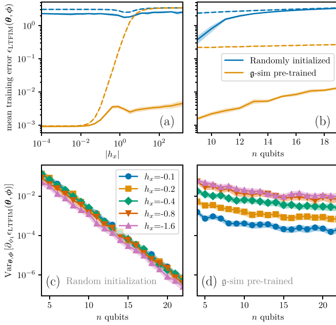
FIG. 5. Pre-training VQE for LTFIM using g-sim. (a), (b) Mean training error \epsilon_{\text{LTFIM}}(\theta, \phi) [Eq. (32)] for VQE with random initialization (blue) and pretrained with g-sim (orange), (a) at n = 12 qubits and varying longitudinal field strengths h_x and (b) at field strength h_x = -1.0 and varying system sizes n . Dashed lines represent initial ansatz configurations, while solid lines represent trained ansätze. (c), (d) Comparison of gradient variances at varying system size n and longitudinal field strengths h_x for (c) uniform random parameter initialization and (d) g-sim pretraining. Shaded bars represent bootstrapped 95% confidence intervals.
