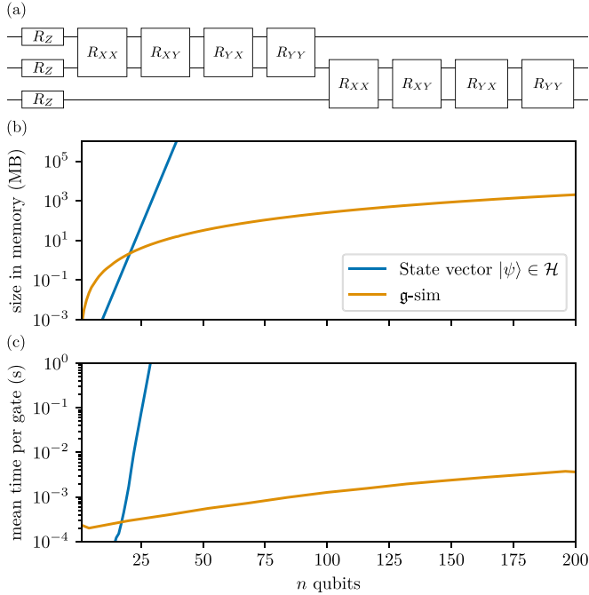
FIG. 3. Performance benchmarks of g-sim. (a) Circuit used for the benchmark at n = 3 qubits. The set of generators is presented in Eq. (22). Here, R_Z denotes a rotation about the Z axis, and R_{\mu\nu} a rotation generated by the Pauli operator \sigma^\mu \sigma^\nu . We compare (b) the memory and (c) compute time requirements for state vector simulations (blue) and g-sim (orange) for the unitary shown in panel (a).
