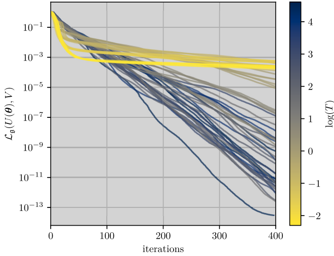
FIG. 12. Compiling short-time dynamics for global Hamiltonians. For a system of n = 20 qubits, we train an overparametrized (27 layer) ansatz to minimize \mathcal{L}_g , with a target unitary generated by a normalized global Hamiltonian. At larger values of T , the expected exponential convergence is observed. At T \approx 1 , a transition is observed to a regime with poorer trainability.
