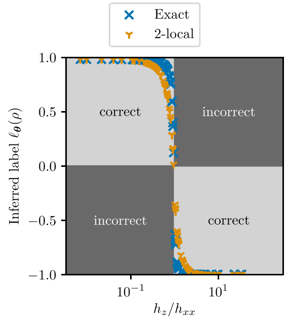
FIG. 13. Comparison of exact label inferences to their 2-local approximation. We compare the exact inferred labels of the TFIM phase classifier on an unseen training dataset to a 2-local approximation. The 2-local approximation still achieves 100% classification accuracy, although \ell_\theta(\rho) changes less rapidly near the phase transition.
