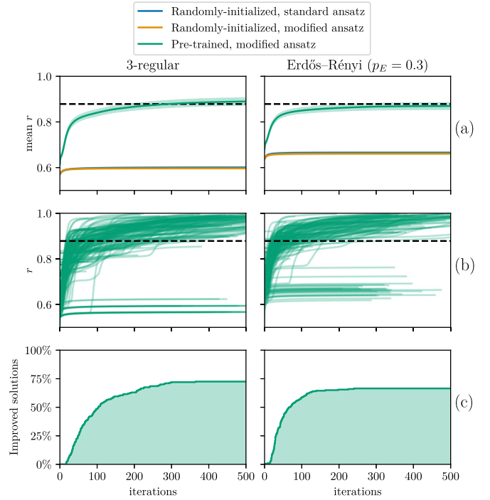
FIG. 6. Pre-training QAOA using g-sim. Performances of QAOA on MaxCut at n = 16 qubits for the standard randomly initialized QAOA ansatz (blue), the modified randomly initialized ansatz (orange), and the modified ansatz pretrained with g-sim (green). Comparisons are made across ensembles of 200 random 3-regular graphs (left panels) and 200 Erdős-Rényi graphs with edge probability p_E = 0.3 (right panels). We compare (a) the mean approximation ratios r (shaded bars are bootstrapped 95% confidence intervals), (b) individual training trajectories, and (c) the fraction of solutions outperforming the GW threshold (reported as a horizontal dashed line).
