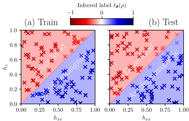
FIG. 10. Supervised QML with a classically efficient circuit. (a) Label assignments from a 50-qubit classifier on a training dataset of disguised TFIM ground states for T = 10 (details in the main text), across the disordered-antiferromagnetic phase transition. The classifier is trained to minimize the loss function in Eq. (44). (b) Inference on a new set of data drawn from the same distribution. The model achieves 100% classification accuracy on the test dataset.
