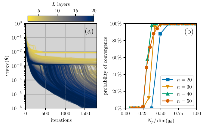
FIG. 4. Overparametrization in large system sizes. (a) Convergence traces at n = 50 qubits of the approximate training error \epsilon_{\text{TFXY}}(\theta) . (b) The probability of converging to \epsilon_{\text{TFXY}} < 10^{-4} for uniform random initialization of \theta as measured by 50 samples, at varied circuit depths, with the corresponding number of parameters N_p reported as a fraction of \dim(\mathfrak{g}_0) and for n ranging from 20 to 50 qubits.
