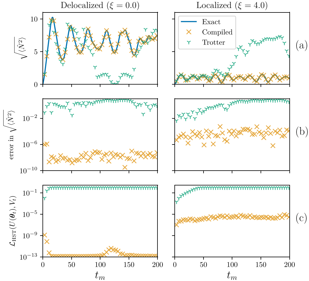
FIG. 9. Compiling Hamiltonian dynamics with g-sim. Dynamics of a single-spin-flip excitation in a TFX spin chain [Eq. (24) with n = 12 ] in the absence of magnetic fields ( \xi = 0 , left panels) and with random fields inducing Anderson localization ( \xi = 4 , right panels). The exact dynamics (blue) is compared with the dynamics yielded by our compilation scheme (orange X), and first-order Trotterization (green Y). The compilation scheme accurately showcases Anderson localization, reproducing the RMS position (\hat{N}^2)^{1/2} of the (a) excitation with (b) low errors, while Trotterization quickly diverges beyond small simulation times. (c) Furthermore, comparison of the compiled unitaries with the exact time-evolution operators by means of the Hilbert-Schmidt test \mathcal{L}_{\text{HST}} shows small errors at all times, guaranteeing faithful dynamics of all observables.
