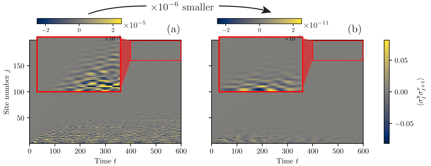
FIG. 2. Noiseless and noisy dynamics of a 200-qubit magic state using g-sim. We simulate the Trotterized dynamics of an initial magic state (25) under a TFXy spin-chain Hamiltonian (24) for n = 200 qubits and \tau = 2.81 in g-sim. We report values for correlators of the form \langle \sigma_j^y \sigma_{j+1}^x \rangle along the dynamics. (a) In the absence of noise, we see that the correlations propagate across the whole chain. This simulation ran in 16 minutes on a single CPU core. The inset shows small oscillations in the correlators that reach the far end of the chain, confirming that the light cone of the dynamics reaches from the first to last qubit. (b) Including noise in the dynamics, in the form of random 2-qubit Pauli channels (26) acting after each entangling gate with a fault probability of p = 3 \times 10^{-4} , we see that the dissipation weakens the correlations by six orders of magnitude.
