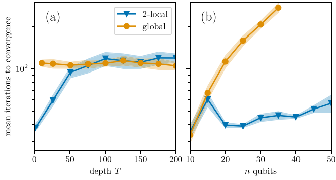
FIG. 7. Scaling properties of circuit compilation with \mathfrak{g} -sim. We compare the mean number of iterations to converge to a loss [defined in Eq. (40)] \mathcal{L}_{\mathfrak{g}} < 10^{-3} for random target unitaries [defined in Eq. (41)] with varied levels of locality, including 2-local and global generators. Results for (a) varying duration T at n = 20 qubits, and for (b) varying system size n at duration T = 10 . The Shaded bars depict bootstrapped 95% confidence intervals. The scaling of the iteration number is found to be polynomial in n and T .
