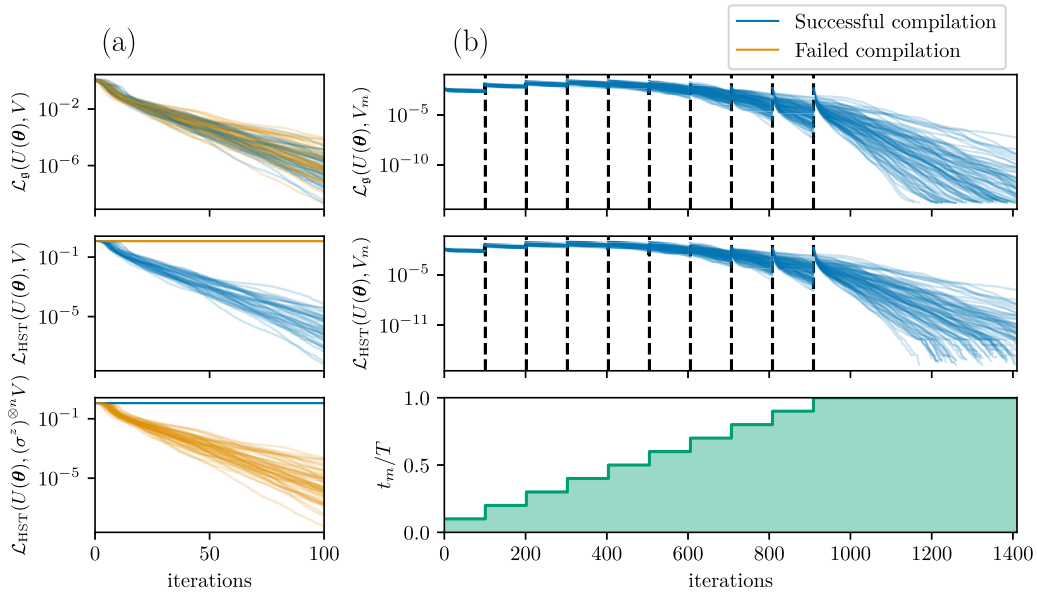
FIG. 8. Successfully compiling circuits in an algebra with nontrivial group center elements. (a) Although the classical loss function \mathcal{L}_{\mathfrak{g}}(U(\theta), V) can be efficiently minimized (Fig. 7), this is a necessary but insufficient condition to minimize the Hilbert-Schmidt loss function \mathcal{L}_{\text{HST}} , and thus to faithfully compile a target unitary V . We train a linear-depth ansatz U(\theta) [see Fig. 3(a)] initialized with uniform random parameters to minimize \mathcal{L}_{\mathfrak{g}}(U(\theta), V) at T = 1 and n = 10 . Although \mathcal{L}_{\mathfrak{g}} is successfully minimized in all instances (top panel), \mathcal{L}_{\text{HST}} is only minimized in approximately half the instances, and rather maximized otherwise (middle panel). In all cases where the compilation fails, the optimized ansatz instead approximates (\sigma^z)^{\otimes n}V (bottom panel). (b) The scheme outlined in Sec. IV C 3 successfully rectifies this issue. The ansatz is initialized at \theta = \mathbf{0} and compiled to a sequence of intermediate targets V_m corresponding to increasing t_m from 0 to T (bottom panel), with the parameters obtained from compiling a target used to initialize the next. For sufficiently small time steps \Delta t_m , successfully minimizing \mathcal{L}_{\mathfrak{g}} (top panel) ensures minimization of \mathcal{L}_{\text{HST}} (middle panel) and thus faithful compilation of the final target V .
