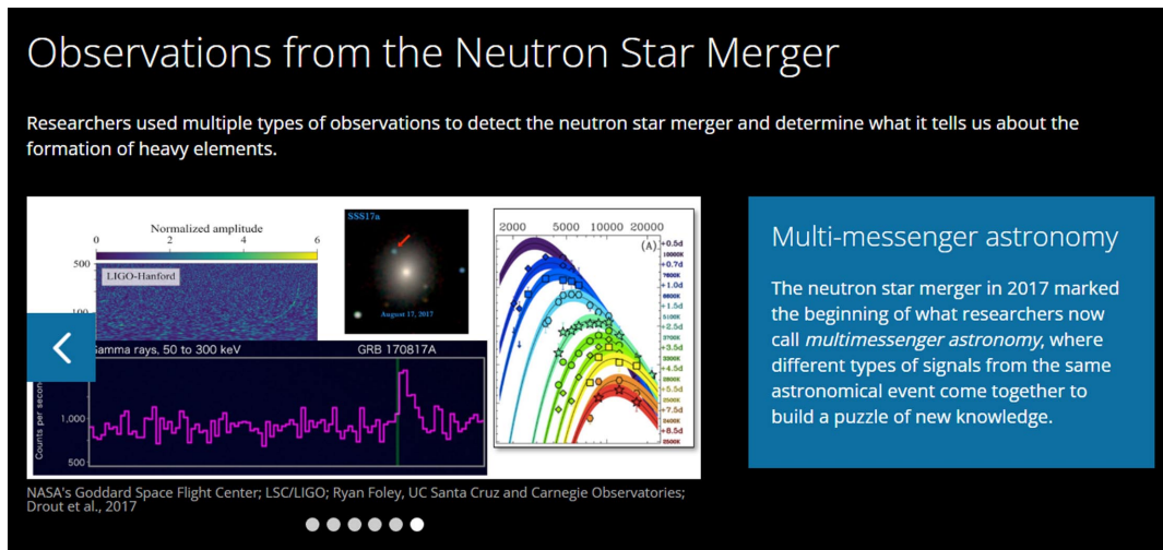
FIG. 5. A sequence of illustrations and texts presents the central observations from the 2017 neutronstar merger and their contributions to new scientific knowledge.
