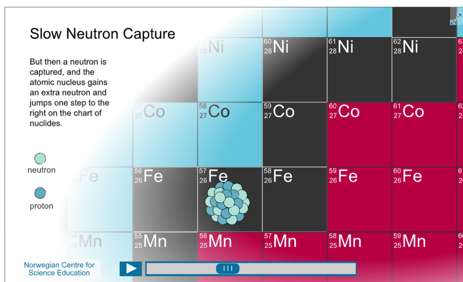
FIG. 4. Interactive animation of the slow neutron capture process; close-up of an area of the chart of nuclides.
