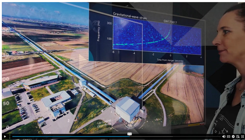
FIG. 2. Screenshot from the video in the beginning of Stars and Elements , showing a gravitational wave detector and the gravitational wave signal (Caltech/MIT/LIGO Lab).
