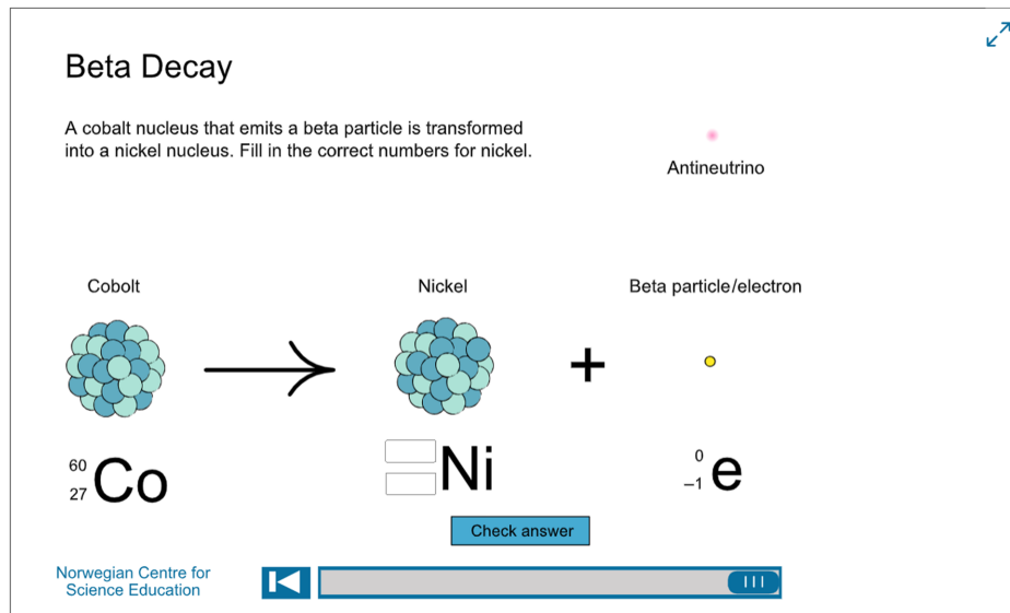
FIG. 3. An interactive animation showing the process of beta decay, asking students to fill in the nucleon and proton number of the daughter nuclide.
