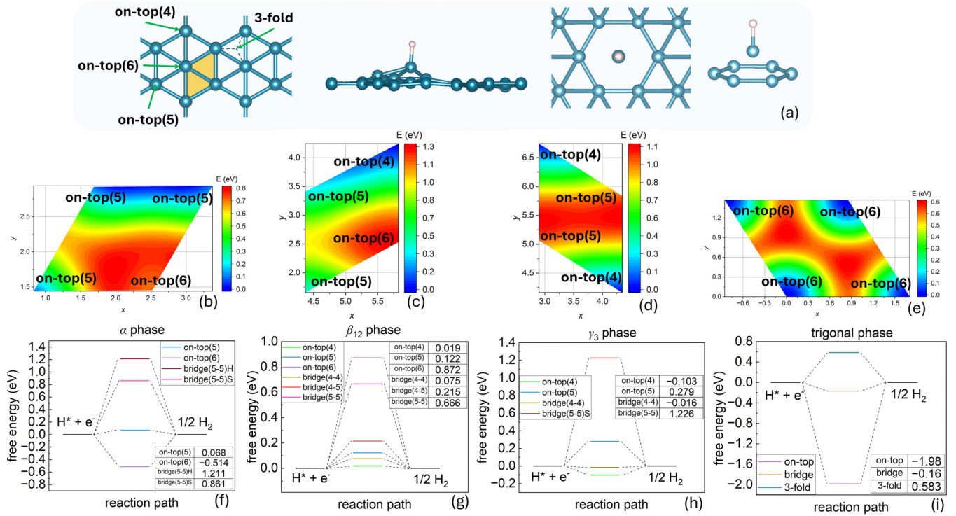
FIG. 2. (a) The leftmost panel illustrates representative adsorption sites on borophene, including on-top( n ) and threefold sites, where n = 4, 5 , or 6 denotes the coordination number of the underlying boron atom (i.e., fourfold, fivefold, and sixfold coordinated sites, respectively). The second panel from the left schematically shows the out-of-plane distortion of the borophene surface upon hydrogen adsorption. The two rightmost panels depict the top and front views of the trigonal phase with H adsorbed at the on-top site; to ensure visual clarity, only the hexagonal ring directly beneath the adsorbed H atom is displayed on the front view. (b)–(e) depict the potential energy surface of single-H adsorption of the four borophene phases: (b) \alpha , (c) \beta_{12} , (d) \gamma_3 , and (e) trigonal. The H atom is moved within a specific region consisting of two adjacent triangular units as highlighted in (a). The distances between H and boron surface are fixed as 1.710, 1.712, 1.690, and 1.760 Å on the \alpha , \beta_{12} , \gamma_3 , and trigonal phases, respectively. The corresponding on-top site types at each vertex are also labeled in each panel. (f)–(i) depict the free energy diagrams for hydrogen adsorption on the \alpha , \beta_{12} , \gamma_3 , and trigonal phases, respectively. Each panel includes a table listing the calculated hydrogen adsorption free energy ( \Delta G_{H^*} ) for the corresponding adsorption sites. In the table, “bridge( m - n )” denotes a bridge site located between two adjacent boron atoms with m - and n -fold coordination. The signs “bridge(5-5)H” and “bridge(5-5)S” in (b) refer to bridge sites located along the edges of hollow hexagons and hexagons containing an additional boron atom at the center, respectively.
