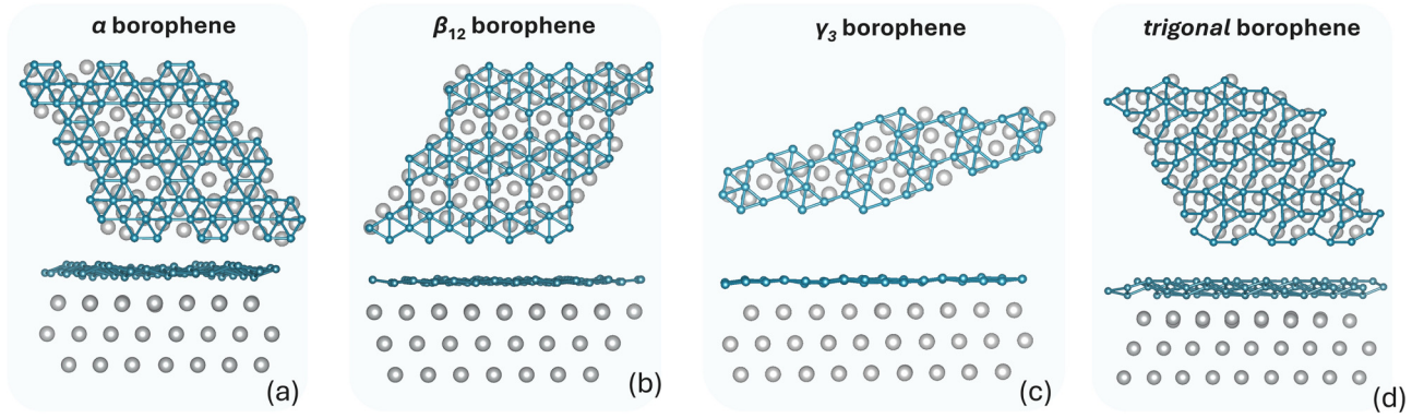
FIG. 3. Optimized structures of borophene phases on the Ag(111) substrate: (a) \alpha , (b) \beta_{12} , (c) \gamma_3 , and (d) trigonal phases. For each configuration, the upper panel shows the top view and the lower panel displays the side view, highlighting the interfacial interaction and structural deformation upon adsorption.
