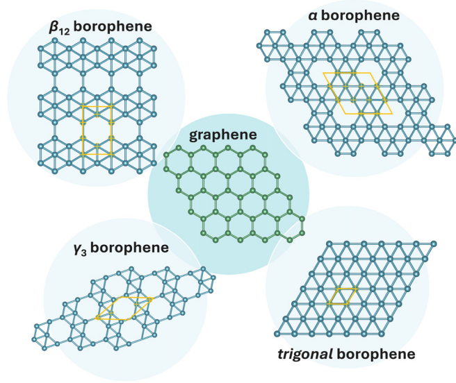
FIG. 1. Geometric configurations of graphene (center panel) and four freestanding borophenes. The structures shown from left to right and top to bottom correspond to the \beta_{12} , \alpha , \gamma_3 , and trigonal phases, respectively. The primitive unit cell of each phase is highlighted in yellow line.
