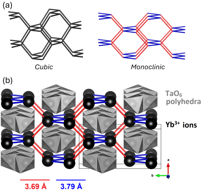
FIG. 1. (a) Schematic illustrating the cubic diamond lattice (all nearest-neighbor distances are equal, shown as black lines) and the “stretched diamond lattice” in monoclinic systems (inequivalent distances between neighboring points, shown as red and blue lines). (b) Crystal structure of M\text{-YbTaO}_4 , space group I2/a (no. 15). \text{Yb}^{3+} ions are shown in black and \text{Ta}^{5+} ions in gray; oxide ions are located at the vertices of the \text{TaO}_6 polyhedra. The red and blue solid lines indicate the two closest Yb–Yb distances making up the stretched diamond lattice.
