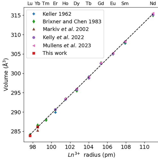
FIG. 3. Unit cell volume of M - Ln TaO 4 compounds [23,26,27,36,42] as a function of lanthanide ionic radius [43].
