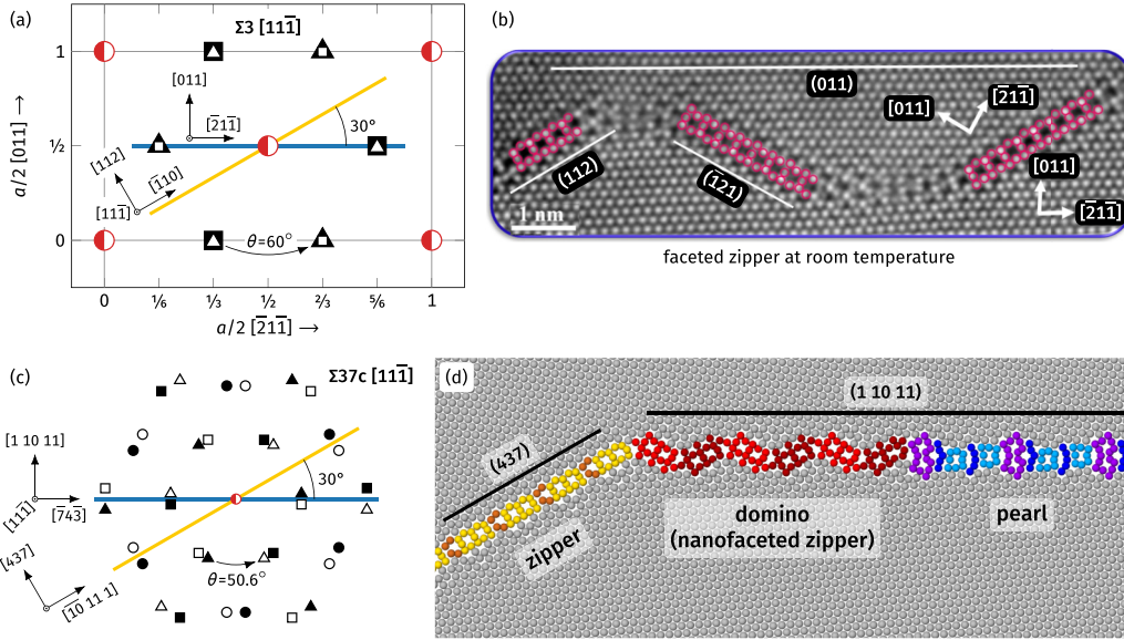
FIG. 1. (a) Dichromatic pattern of \Sigma 3 [11\bar{1}] tilt GBs. Black and white symbols represent the atoms of the two crystallites, while the shape of the symbols represents the different (11\bar{1}) planes on which these atoms lie. The black and white symbols coincide in the projection, but are located on different planes. The red data points are coincidence sites. The crystal directions refer to the coordinate system of the lower crystallite. Two possible (quasi)symmetric GB planes are indicated. (b) At room temperature, faceted zipper structures were observed experimentally in Al on \{112\} planes. The structure on the (011) plane is not reported in the literature. Image from Ref. [35] with crystallographic directions and planes adjusted to the convention of the present paper. Reused under the terms of the Creative Commons Attribution 4.0 International license. (c) Excerpt of the dichromatic pattern of a \Sigma 37c [11\bar{1}] tilt GB. The red data point is a coincidence site. The full dichromatic pattern can, for example, be found in the Supplemental Material of Ref. [32]. (d) Snapshot of a simulation of the corresponding GB phases. The domino phase consists of nanoscale facets of zipper structures [15]. This nanofaceting is impossible in the \Sigma 3 GB, where the facets are energetically driven to grow [15]. We hypothesize that pearl-like phases may exist on the (011) plane of \Sigma 3 .
