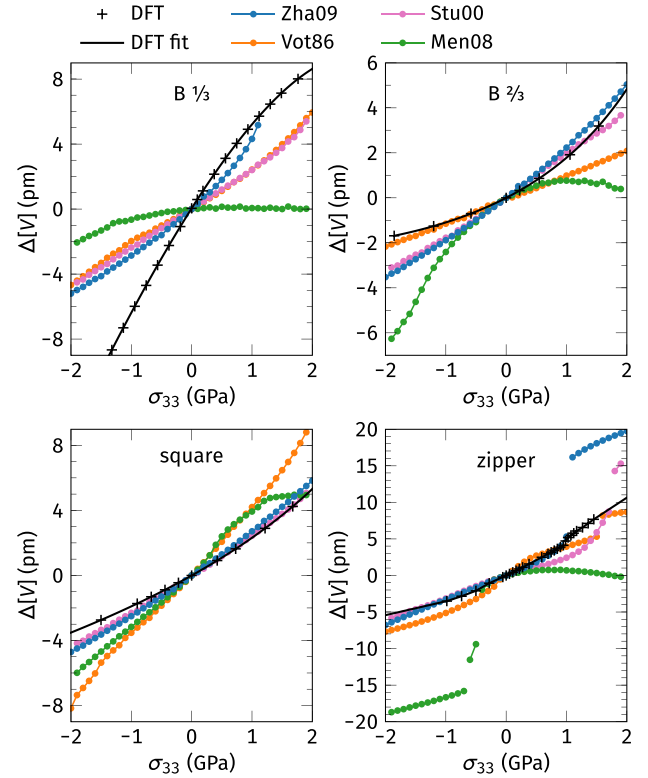
FIG. 10. Change of excess volume with applied stress \sigma_{33} . For DFT, the data points represent individual calculations and the lines are polynomial fits to the data.
