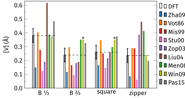
FIG. 8. Comparison between excess volumes calculated with DFT and with empirical potentials. The DFT error bars are conservatively estimated to be \pm 0.05 Å from variations in the GB energy with system size during convergence studies (Figs. S7–S9 within the SM [55]). The B 2/3 structure minimized with the Win09 potential (marked by an asterisk) transforms into the square structure.
