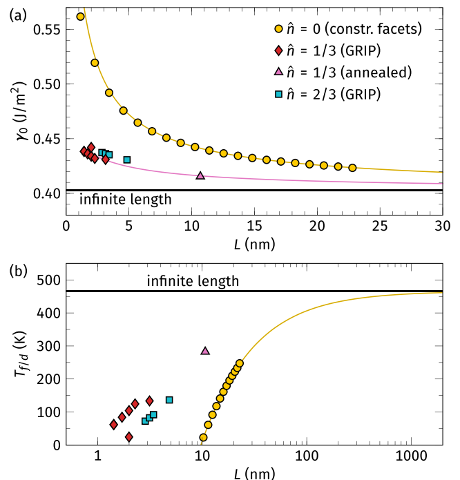
FIG. 4. Influence of the finite length of \{112\} facets located on an average (011) GB plane. (a) Ground-state energy \gamma_0 of faceted zipper GBs as a function of facet length L . Differences in energy, especially at small L , are the result of different facet-junction energies as a function of \hat{n} . The lines represent a fit of Eq. (10) to the data. Data points for \hat{n} = 0 were constructed by joining zipper facets as described in Ref. [15]. For \hat{n} = 1/3 and 2/3 , the structures were obtained with GRIP. We replicated one sample with \hat{n} = 1/3 along the y direction and annealed it to obtain longer facet lengths. (b) By adding the facet-junction energies to the excess free energies from Fig. 3(a), we can estimate the change of the transition temperature T_{f/d} for different facet lengths.
