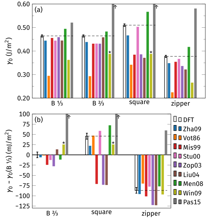
FIG. 7. (a) Comparison between GB energies calculated with DFT and with empirical potentials. The DFT error bars are conservatively estimated to be \pm 5 \text{ mJ/m}^2 = \pm 0.3 \text{ meV}/\text{\AA}^2 from variations in the GB energy with system size during convergence studies (Figs. S7–S9 within the SM [55]). The B 2/3 structure minimized with the Win09 potential (marked by an asterisk) transforms into the square structure. (b) GB energy difference compared to B 1/3.
