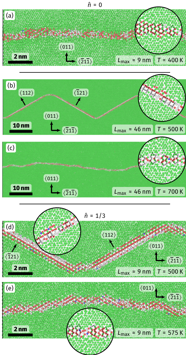
FIG. 5. Snapshots from MD simulations of \Sigma 3 [11\bar{1}] (011) GBs. (a) A GB with \hat{n} = 0 does not exhibit any faceting. Here, the simulation cell size admits a maximum facet length of L_{\max} = 9 nm and therefore the facet junction energy is too high (see also Fig. 4). (b), (c) When allowing facet lengths up to 46 nm, a transition can be observed. (d), (e) For \hat{n} = 1/3 , the facet junction energies are lower. We observe faceting up to 500 K (d), while a rough but flat GB occurs at 575 K and above (e). In between, we observe a mix. The round insets show a zoom onto a slice with a thickness of 3 atomic layers, which allows to identify the atomic motifs of the GB. We find zipper structures in the faceted GBs and B structures in the flat GBs. Indicated crystal directions refer to the lower crystallite. Equivalent crystal directions according to the misorientation in the upper crystallite not shown.
