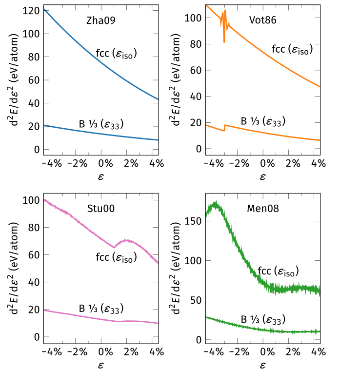
FIG. 11. Second derivative of the potential energy with strain, computed using finite differences. For each potential, both an fcc unit cell and a B 1/3 GB were strained; fcc hydrostatically and the GB along the z direction. These plots reveal numerical problems with cutoffs, noise, and fluctuating curvature of the empirical potentials.
