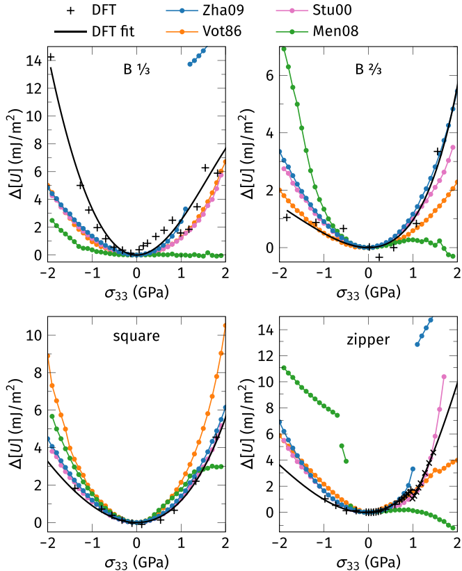
FIG. 9. Change of excess energy with applied stress \sigma_{33} . For DFT, the data points represent individual calculations and the lines are polynomial fits to the data.
