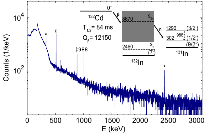
FIG. 1. Gamma spectrum following the decay of ^{132}\text{Cd} . We observe no gamma transitions in ^{131}\text{In} and just one transition in ^{131}\text{In} at 988 keV, populated after beta-delayed neutron emission [19]. We observe two transitions following the decay of ^{131}\text{In} (*), and a variety of background lines corresponding to neutron scattering in Ge(†), ^{84}\text{Rb} contamination from a previous experiment (‡), and the 511 keV positron annihilation line (§). The top right inset shows a schematic of the ^{132}\text{Cd} beta decay.
