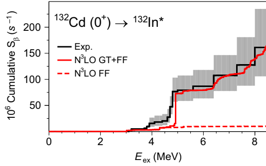
FIG. 3. Cumulative decay strength as a function of the excitation energy in ^{132}\text{In} . We obtained the strength using the intensities from the fit of the neutron time-of-flight spectrum (Fig. 2), the total number of ^{132}\text{Cd} decays ( 2.2 \times 10^5 ), and assuming a neutron branching ratio of 100%. The large jump in strength at around 5 MeV corresponds to the most intense neutron transitions observed at 2 MeV in Fig. 2. The red line corresponds to the total decay strength calculated using the LSSM with \text{N}^3\text{LO} [15], while the dashed red line is just the FF strength. The model reproduces very well the experimental decay strength, further supporting its consistency across N = 82, 84 nuclei with Z < 50 .
