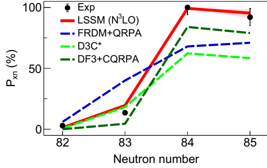
FIG. 5. Beta-delayed neutron branching ratios of N = 82 to N = 85 cadmium isotopes [38], compared to the model using LSSM with N^3\text{LO} (red). For comparison, we show neutron branching ratios from FRDM-QRPA [9] (dashed teal), DF3-CQRPA [10] (dashed dark green), and D3C* [33] (dashed green). While the LSSM with N^3\text{LO} calculation reproduces well all neutron branching ratios, all “global models” substantially underpredict ^{132,133}\text{Cd} .
