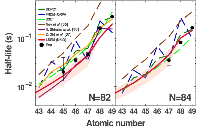
FIG. 4. Left: decay half-lives of N = 82 isotones ([38]) compared with our calculation using LSSM with \text{N}^3\text{LO} (red). The uncertainty band in light red corresponds to changing the unknown Q_\beta values by \pm 0.5 MeV. We include calculations using FRDM-QRPA [9] (dashed dark blue), D3C* [33] (dashed green), DDPC1 [34] (dashed dark green), Ney et al. [35] (dashed brown), and shell model calculations from Shimizu et al. [36] (purple) and Zhi et al. [37] (orange). Right panel: same for N = 84 isotones. Note that prior to our model no other LSSM calculations were available. In both cases we see that experimental values are well reproduced by models except of Ney et al. and FRDM-QRPA, the latter being the leading model used in r -process calculations [1,2]. The “seesaw” behavior of FRDM-QRPA half-lives is driven by their treatment of pairing in their mass and Q_\beta calculations, resulting in larger half-lives of the important even-even nuclei [1].
