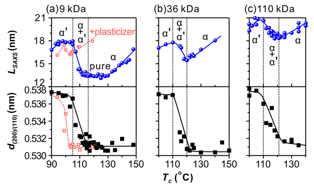
FIG. 2. X-ray data for the three polymers as a function of T_c . Top: SAXS long period. Bottom: 110/200 WAXS lattice spacing. (a) PLLA-9K, (b) PLLA-36k, and (c) PLLA-110K. The data for plasticized PLLA-9k are shown as red empty circles in (a). All the samples were crystallized isothermally in DSC apparatus, then quenched at room temperature, recorded at room temperature. Raw SAXS/WAXS data are at [24].
