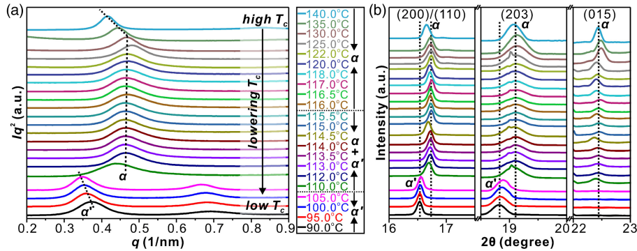
FIG. 5. (a) and (b) are ex situ SAXS and WAXS profiles of PLLA-9k isothermally crystallized at different temperatures, as indicated.
