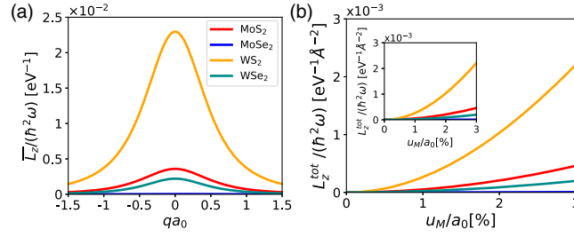
FIG. 1. Electronic OAM induced by the phonon at K point with l_{\text{ph}} = 1 in monolayer TMDs MoS 2 , MoSe 2 , WS 2 , and WSe 2 . (a) OAM as a function of wave number q with u_M/a_0 = 1\% . (b) Total OAM as a function of u_M/a_0 .
