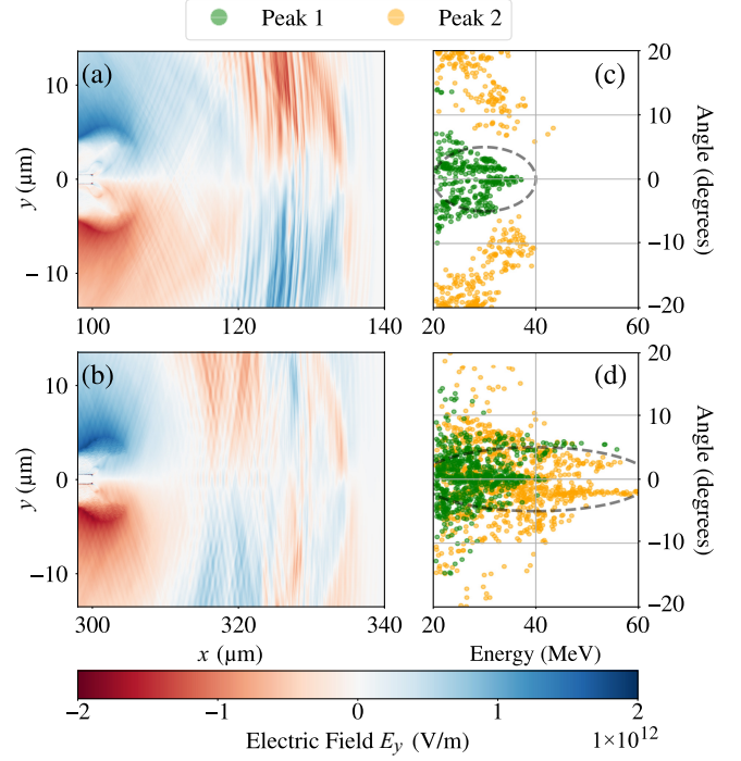
FIG. 4. Cycle averaged electric field component E_y with tracked electrons. (a) 100 \mu\text{m} target at 530 fs. (b) 300 \mu\text{m} target at 1200 fs. (c), (d) Indicate the angular distribution of electrons selected from Peak 1 and Peak 2 at 400 fs indicated in Fig. 3(b). Dashed ellipses show electrons that would be detected on Espec 0.
