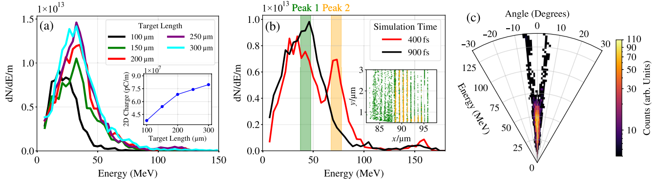
FIG. 3. (a) 2D simulated electron spectra at different values of target lengths taken 100 fs after exiting into vacuum. Particles were selected within a 20 \mu\text{m} slice. The inset shows the linear electron charge density vs target length. (b) Energy spectrum of electrons selected within the final spectrum for 250 \mu\text{m} target at 400 fs and 900 fs, respectively. Peaks 1 and 2 indicate electrons selected at 400 fs for Fig. 4, with an inset showing these electrons trapped in an SPW. (c) Polar plot of the angular distribution of the tracked electrons emitted from the rear edge of a 250 \mu\text{m} target.
