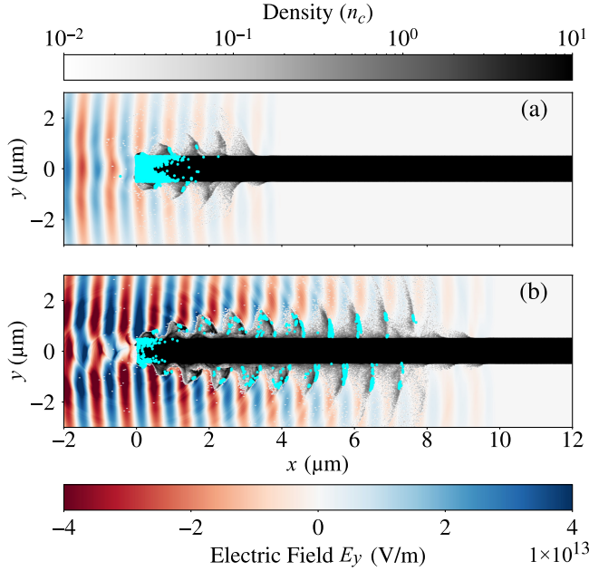
FIG. 5. Particle tracking simulation snapshots of a parallel laser-solid interaction, showing the tracked electrons from the spectrum in Fig. 3(a) (cyan) overlaid with the electric field component E_y and electron density (gray) at times (a) t = 80 fs and (b) t = 100 fs.
