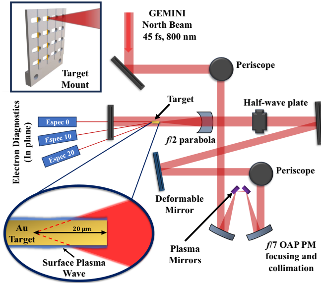
FIG. 1. Schematic of the experimental setup. Three high-resolution electron spectrometers were deployed at different angles 0^\circ , 10^\circ , and 20^\circ (as labeled) with respect to the target surface. The bottom inset depicts the irradiating position with the laser pulse focused 20\ \mu\text{m} beyond the front edge of a 6\ \mu\text{m} gold target. The top inset shows the target matrix array used for parallel incidence shots.
