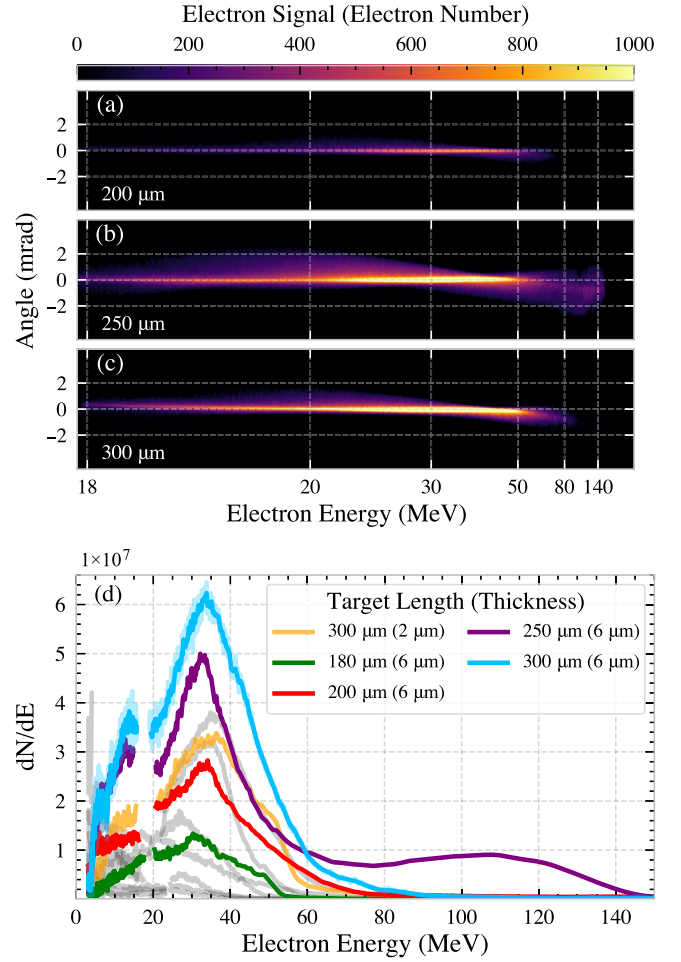
FIG. 2. (a)–(c) Raw BAS-TR image plate data from Especc 0 degrees. Electrons are generated from gold foils irradiated at parallel incidence using 200, 250, and 300\ \mu\text{m} targets, respectively. (d) Electron spectra at 0^\circ , smoothed using a 6\sigma Gaussian filter. Several representative shots for target lengths ranging from 180 to 300\ \mu\text{m} are highlighted, while others are plotted in light gray to indicate shot-to-shot variations. Gaps around 17 MeV correspond to the electron spectrometer arrangement, specifically the separation between two image plates.
