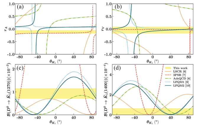
FIG. 3. Comparisons of (a) r_A , (b) r_V , (c) \mathcal{B}[D^0 \rightarrow \bar{K}_1(1270)^- e^+ \nu_e] , and (d) \mathcal{B}[D^0 \rightarrow \bar{K}_1(1400)^- e^+ \nu_e] measured in this Letter and predicted by various theoretical approaches as a function of \theta_{K_1} . The yellow bands show \pm 5\sigma limit for (a), (b), (c), and the upper limit at 90% CL for (d).
