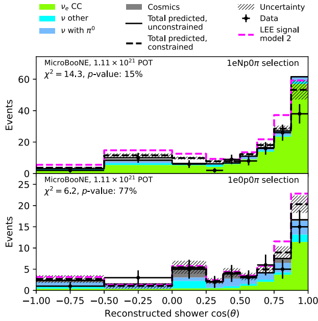
FIG. 4. Distribution of MC simulation compared with data for reconstructed shower \cos(\theta) in the 1eNp0\pi and 1e0p0\pi signal channels, along with the LEE Signal Model 2 .
