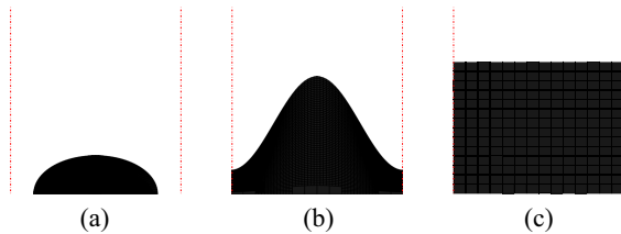
FIG. 1. A schematic drawing of the transverse horizon radius for different black hole phases with standard Kaluza-Klein asymptotics: (a) the localized black hole phase, (b) the nonuniform string phase, and (c) the uniform string phase.
