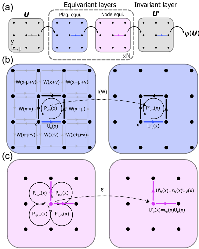
FIG. 1. Example configuration of the LGNWF ansatz. (a) Schematic of updating a lattice of links, U , through N blocks of equivariant layer-to-layer transforms (b) and (c). (b) Plaquette equivariant network updating the link U_\mu(x) through Eqs. (6) and (7) conditioned on nonlocal information W . (c) Node equivariant layer acting on U_\mu(x) and U_\nu(x) through Eqs. (8) and (9), acting only on plaquettes originating at x .
