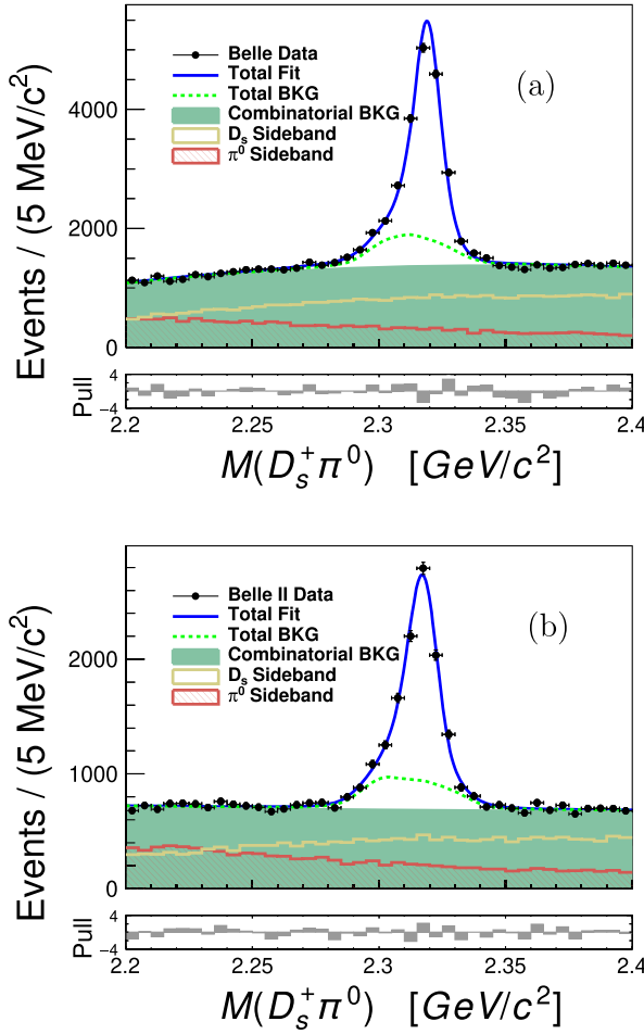
FIG. 1. Invariant mass distributions of D_s^+ \pi^0 from (a) Belle and (b) Belle II data. The data samples are represented by the dots with error bars. The blue curves, green dotted curves, and green filled areas are the fitted total PDFs, total backgrounds, and combinatorial backgrounds, respectively. The areas between total and combinatorial backgrounds are from the fitted cross-feed contributions. The distributions from the normalized D_s^+ and \pi^0 mass sidebands are shown with yellow blank and red slash filled histograms, respectively.
