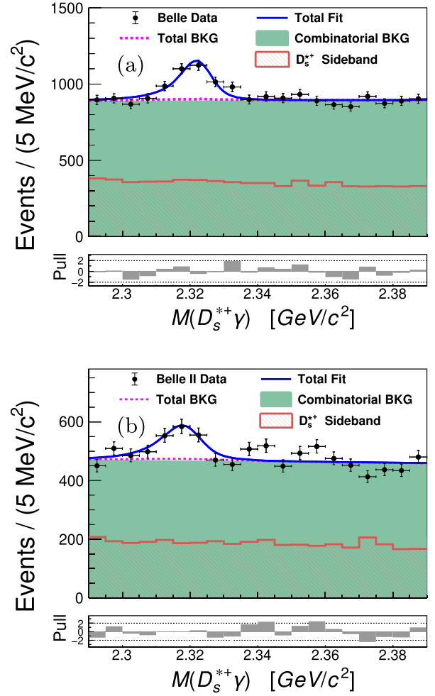
FIG. 2. Simultaneous fits to the M(D_s^{*+} \gamma) distributions from (a) Belle and (b) Belle II. The blue and violet curves are the best fit results and the fitted total background PDFs, respectively. The filled green areas are the fitted combinatorial backgrounds. The histograms in red slashes represent the normalized D_s^{*+} sidebands.
