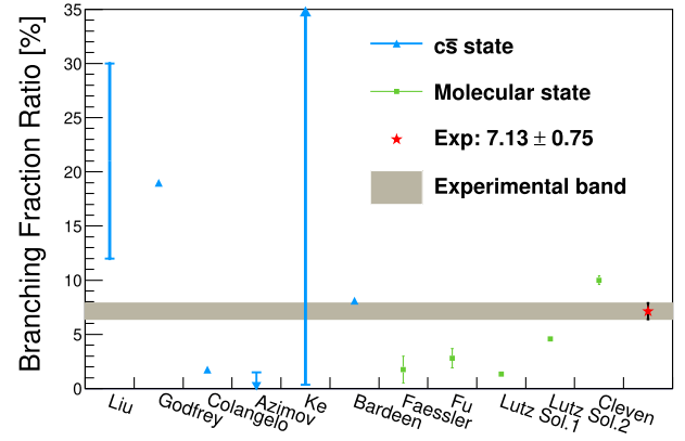
FIG. 3. Comparison of the measured \mathcal{B}[D_{s0}^*(2317)^+ \rightarrow D_s^{*+}\gamma]/\mathcal{B}[D_{s0}^*(2317)^+ \rightarrow D_s^{*+}\pi^0] with theoretical predictions. The theoretical approaches of the references are effective field theory for Liu [26] and Cleven [11], traditional quark model for Godfrey [48], heavy quark symmetries for Colangelo [24], phenomenological for Azimov [25], light front quark model for Ke [71], effective Lagrangian with chiral symmetry for Bardeen [21], effective Lagrangian for Faessler [45], heavy quark flavor symmetry for Fu [46], and chiral Lagrangian with coupled-channel dynamics for Lutz [47]. The prediction of Ke [71] is a lower limit indicated by an arrow. The uncertainty of the experimental measurement is the quadrature sum of statistical and systematic uncertainties.
