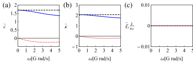
FIG. 3. Effective properties of a symmetric trilayer made of a diamond layer in-between two SiO 2 layers [Fig. 1(b)]. Legend as in Fig. 2. The bianisotropic terms are null, owing to the symmetry of the scatterer.
