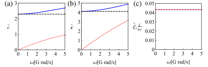
FIG. 4. Effective properties of a trilayer made of SiO 2 , diamond and copper layers [Fig. 1(c)]. Legend as in Fig. 2.
