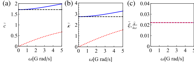
FIG. 2. Effective (a) specific heat and (b) thermal conductivity properties of a bilayer made of SiO 2 and diamond [Fig. 1(a)]. Solid blue and dashed red curves denote real and imaginary parts, respectively. Dashed black lines denote the harmonic and arithmetic means. (c) Effective bianisotropic terms \tilde{\xi} (dashed red) and \tilde{\chi}/i\omega (solid blue).
