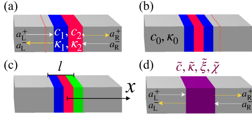
FIG. 1. Heterogeneous scatterers in between two homogeneous semi-infinite slabs. (a) Bilayer scatterer. (b) A symmetric trilayer scatterer. (c) Asymmetric trilayer. Red lines in panels (a) and (b) denote planar heat sources at the left and right slabs. (d) Homogeneous scatterer with effective bianisotropic terms that generates that same scattering response as the heterogeneous scatterer.
