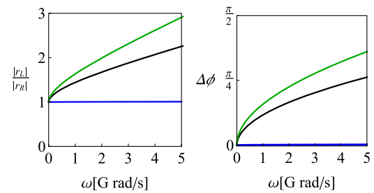
FIG. 5. Magnitude ratio (left panel) and phase difference (right panel curves) between the reflection coefficients ( r_L and r_R ) as functions of frequency, for the different scatterers shown in Figs. 2 (black), 3 (blue), and 4 (green).
