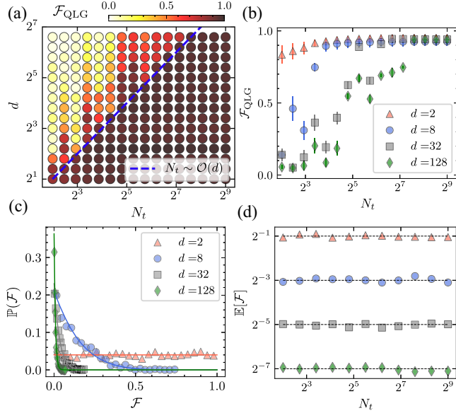
FIG. 2. Haar-random state benchmark. (a) Average fidelity \mathcal{F}_{\text{QLG}} \equiv |\langle \psi_{\text{QLG}} | \psi_{\text{Haar}} \rangle|^2 of Haar-state preparation versus Trotter depth N_t and Hilbert subspace dimension d , where each marker is averaged over 10^2 randomly sampled Haar unitaries. The blue dashed line indicates the empirical scaling N_t \sim \mathcal{O}(d) required to reach high fidelity ( \mathcal{F}_{\text{QLG}} \gtrsim 0.95 ). (b) Fidelity \mathcal{F}_{\text{QLG}} versus N_t for different dimensions d ( 10^3 samples per point). (c) Probability density distribution \mathbb{P}(\mathcal{F}) of the stochastic fidelity \mathcal{F} = |\langle \psi_{\text{QLG}} | \psi_{\text{ref}} \rangle|^2 over 10^2 \times d QLG realizations (markers) compared with the analytical Haar statistics \mathbb{P}_{\text{Haar}}(\mathcal{F}) given by Eq. (10) (solid curves) for different dimensions. (d) Mean fidelity \mathbb{E}[\mathcal{F}] versus N_t , with the theoretical prediction 1/d shown as dashed lines. Other parameters are the same as in Fig. 1.
