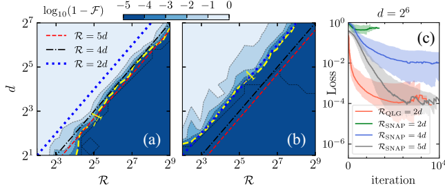
FIG. 4. Controllability benchmark. Average infidelity for preparing 10^2 Haar-random target states as a function of the Hilbert-space dimension d and the number of trainable parameters \mathcal{R} . Results for the SNAP- and QLG-based circuits are shown in panels (a) and (b), respectively. The thick yellow dashed curve marks the contour \log_{10}(1 - \mathcal{F}) \simeq -4 , while the other dotted and dashed guide lines indicate linear scalings \mathcal{R} = 2d, 4d, 5d . (c) Training dynamics for d = 2^6 , showing the loss versus iteration under the same optimization setup for several parameter budgets. Parameters: \delta = 2 and \alpha_{\max} = \sqrt{d} .
