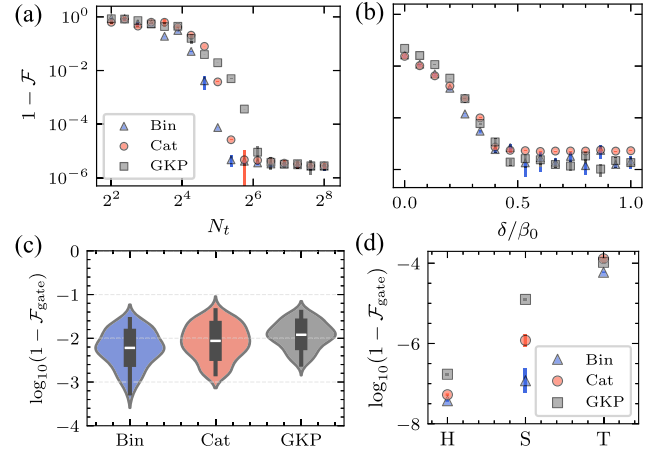
FIG. 3. Bosonic code preparation and operation. (a),(b): Infidelity of prepared code states versus (a) Trotter depth N_t and (b) control bound \delta/\beta_0 for the binomial (triangle), cat (circle), and GKP (square) codes. (c) Violin plots for the binomial (Bin), Cat, and GKP codes by randomly sampling over 10^2 logical gates. The width of each violin (colored region) for a given infidelity logarithm value \log_{10}(1 - \mathcal{F}_{\text{gate}}) is proportional to the probability density of the infidelity. The white line marks the median and the black box represents the interquartile range. (d) Infidelity of elementary single-qubit gates \{H, S, T\} realized via quantum optimal control for each code. The error bars indicate standard deviation over 10^2 data points. Parameters: \delta = 1 for (a), N_t = 2^6 for (b), and N_t = 2^8 , \delta = 2 for (c),(d). Other parameters follow Fig. 1.
