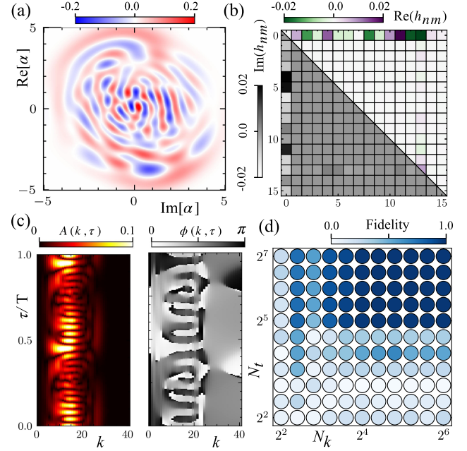
FIG. 1. Single-period Floquet control with QLGs. (a) Wigner function of the target state |\psi_{\text{tar}}\rangle . (b) Target Hamiltonian \hat{H}_{\text{tar}} = i\lambda \log(\hat{U}_{\text{tar}}) in the Fock basis, where the target unitary \hat{U}_{\text{tar}} is constructed from Eq. (9). (c) Amplitude A(k, \tau) and phase \phi(k, \tau) of the driving potential over one Floquet period T . (d) State-preparation fidelity \mathcal{F} = |\langle \psi_{\text{tar}} | \hat{U}_{\text{tar}} | \psi_0 \rangle|^2 as a function of Trotter depths N_k and N_t . We use N_t = 2^6 and N_k = 40 in (a)–(c). Other parameters: N_p = 15 , k_f = 40 , and \beta_0 = 1 .
