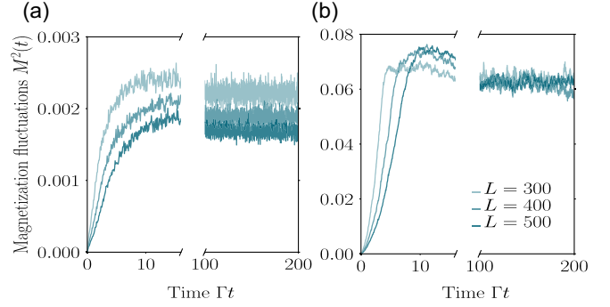
FIG. 4. Classical analog of the quantum flocking problem. Dynamics of magnetization fluctuations M^2(t) for the alignment parameter K = 0.5 in (a) and K = 3.5 in (b).
