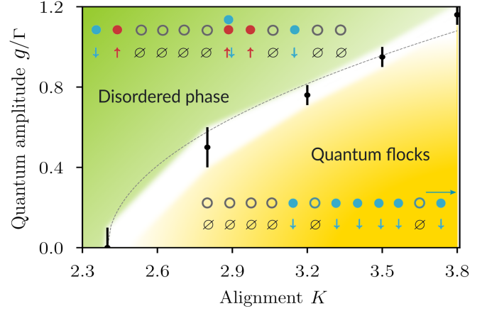
FIG. 2. Phase diagram. Numerically obtained phase diagram with indicated error bars as a function of the alignment parameter K and the quantum amplitude g including representative many-body configurations. The numerical uncertainty for the estimate of the phase transition points is indicated by the white region separating the disordered from the quantum flocking phase. The analytical prediction from the coarse-grained theory at weak quantum amplitudes g is included as a dashed line, which is consistent with the numerical results.
