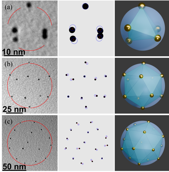
FIG. 2. Experimental imprints and projected Thomson configurations for small charged helium nanodroplets. TEM images of imprints containing N = 5 (a), 11 (b), and 16 (c) singly charged Au-NPs are shown from top to bottom. The left column shows the TEM image of each imprint, with the reconstructed droplet boundary indicated by a red circle. The middle column compares the experimentally determined nanoparticle centroids (black dots) with the best-fitting orthographic projection of the corresponding ideal Thomson configuration (open blue circles). The right panel displays a three-dimensional rendering of the same Thomson configuration.
