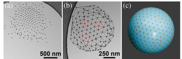
FIG. 3. Local hexagonal order and topological defects in large-droplet imprints. (a) TEM imprint of a large helium droplet with a radius of about 1 \mu\text{m} . Extracted particle positions are overlaid as enlarged black dots. The particle density decreases toward the imprint periphery, resulting in a washed-out outer region. (b) Hemispherical experimental imprint in the range of 375 < r < 600 nm. Neighboring particles are connected via triangulated edges to visualize the local hexagonal order. Red pentagons mark fivefold disclinations. (c) Rendering of an ideal Thomson configuration with 400 singly charged Au-NPs, shown as an orthographic projection of the visible hemisphere.
