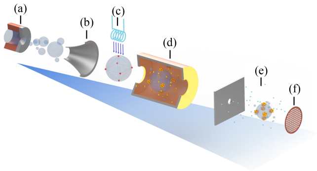
FIG. 1. Schematic of the experimental setup. (a) Pinhole nozzle for supersonic expansion of pre-cooled helium gas into vacuum. (b) Conical skimmer selecting the central HND-beam portion. (c) Nier-type electron impact source. (d) Resistively heated crucible containing Au vapor. (e) Shrinking of HNDs via collisions with room-temperature helium gas. (f) TEM grid to deposit the Au-NPs.
