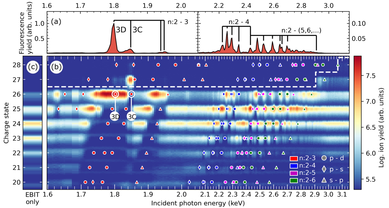
FIG. 3. Overview spectrum from 1.6 to 3.1 keV with highly charged krypton in EBIT. (a) Fluorescence yield; (b) charge-state distribution (CSD) versus incident photon energy; (c) initial CSD without XFEL irradiation. Note the change in the scaling of the photon-energy axis around 2.1 keV. Predicted energies of major ground-state transitions for each charge state are marked with colors according to the upper state n and symbols for the orbital angular momentum, e.g., blue circles for 2p \rightarrow 4d transitions. The white dashed line marks the ionization threshold.
