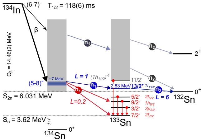
FIG. 2. Schematic decay scheme of ^{134}\text{In} emphasizing \beta n feeding to the i_{13/2} s.p. orbital in ^{133}\text{Sn} . The GT transitions from ^{134}\text{In} strongly populate \sim 7 MeV excitations in ^{134}\text{Sn} [7]. First neutrons ( n_1 ) emitted from these excitations populate bound- and unbound-neutron states in ^{133}\text{Sn} . The highlighted n_1 emission feeds the i_{13/2} neutron state between the known 2f_{5/2} s.p. state and the 1h_{11/2} neutron-hole state in ^{133}\text{Sn} . This state decays exclusively to the ^{132}\text{Sn} ground state through second-neutron ( n_2 ) emission; see text.
