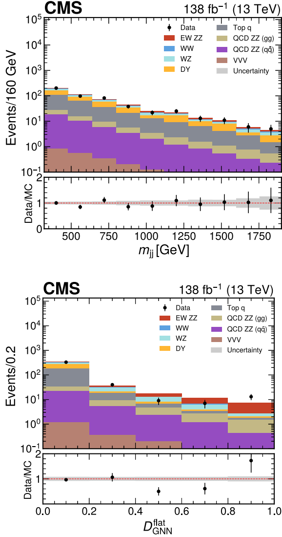
FIG. 2. Distributions of the dijet invariant mass (upper) and the flattened GNN discriminator (lower) in the SR after the maximum likelihood fit. The data are shown as black points, whereas the stacked histograms represent the fitted signal and background contributions. The vertical bars on the data points represent the statistical uncertainties. The gray band indicates the total uncertainty in the prediction after the fit, including both statistical and systematic components.
