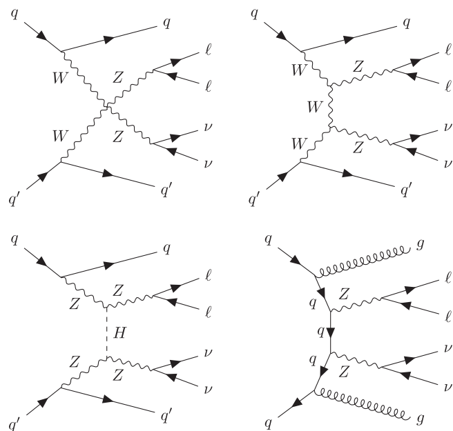
FIG. 1. Example Feynman diagrams of the signal EW ZZ process (first three diagrams) and the QCD ZZ ( q\bar{q} ) background process (last diagram).
