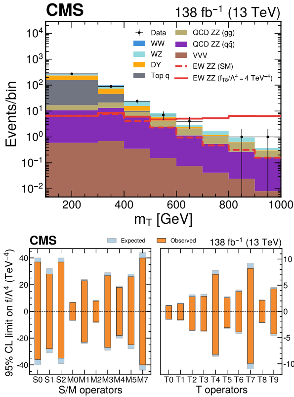
FIG. 3. The m_T distribution (upper) with the expected contribution from a T8 operator, showing the SM case with all EFT Wilson coefficients set to zero (dashed red), and the case with f_{T8}/\Lambda^4 = 4 \text{ TeV}^{-4} (solid red). The vertical bars on the data points represent the statistical uncertainties. The expected and observed limits (lower) at 95% CL are obtained from the likelihood fits.
