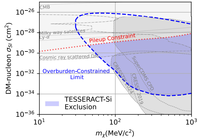
FIG. 5. The 90% CL limits on spin-independent DM below 1 GeV/c 2 . The blue shaded region shows the exclusion from this Letter. The blue dashed line represents the exclusion from the Yellin optimum interval test when considering the effect of the overburden. The red dotted line is from the requirement that there be no DM signal pileup. Previously excluded DM phase space from the CRESST [26,29] and SuperCDMS [25] Collaborations are shown in gray. Constraints from cosmology and astrophysics are shown in light gray [30–34].
