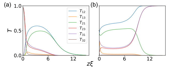
FIG. 2. One channel per terminal. Energy dependence of transmission coefficients for two different choices of time-reversible \hat{s}_{\text{in}} . (a) Realization of the insulating fixed point. (b) Realization of a QTC fixed point. We choose c = 1.5 where both fixed points occur with comparable probabilities.
