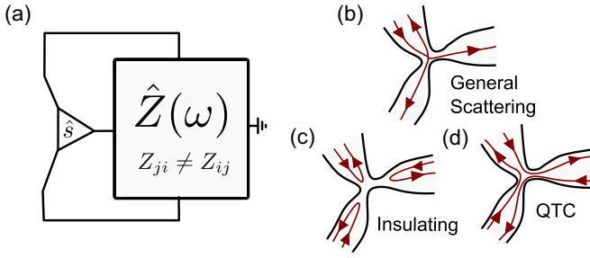
FIG. 1. (a) The N -terminal scatterer ( N = 3 ) embedded in a linear electromagnetic environment which is characterized by the generally nonsymmetric N \times N impedance matrix \hat{Z}(\omega) . (b) Sketch of a general (high-energy) scattering matrix: an incoming electron wave is scattered back and to other terminals. (c) Insulating fixed point: all incoming waves are reflected in the low-energy limit. (d) Predicted QTC fixed point: all incoming waves are fully transmitted to different terminals realizing IQHE phenomenology in the low-energy limit.
