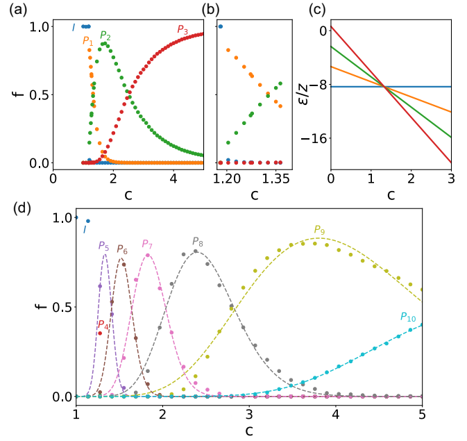
FIG. 4. Three channels per terminal. (a),(b) The probabilities for the realization of QTC fixed points P_n versus c . 10^4 runs per point in c . (b) Close-up the same data as in (a) in the vicinity of c_c . (c) The pseudopotential for P_n and the insulating point. Ten channels per terminal. (d) The probabilities for the realization of QTC fixed points P_n versus c . 10^3 runs per point in c .
