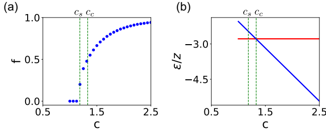
FIG. 3. One channel per terminal. (a) The fraction of \hat{s}_{\text{in}} flowing to QTC fixed point P_1 versus asymmetry parameter c . 10^4 runs per point in c . (b) The pseudopotential \varepsilon of the insulating fixed point (red) and P_1 (blue). c_s , c_c indicate the stability and pseudopotential crossing thresholds, respectively.
