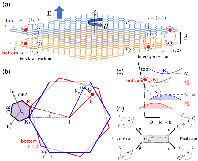
FIG. 1. (a) Sketch of a bilayer system, showing two types of interlayer and intralayer excitons. (b) Brillouin zones of top (blue) and bottom (red) monolayer. Mini Brillouin zones (mBZ) of the moiré bilayer. (c) Sketch of interlayer exciton in momentum space. (d) Diagram of exciton-exciton Coulomb interaction where electron and hole layer indices \ell do not change, and same-layer identical particles can be exchanged.
