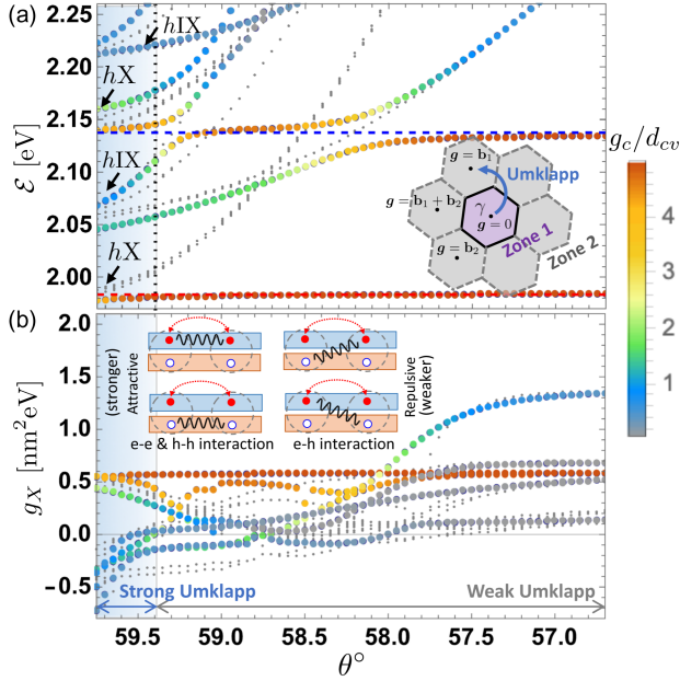
FIG. 2. (a) Exciton energy \mathcal{E}(\sigma = \uparrow) and twisting angle \theta dependence. The points are color coded by its light-matter coupling strength g_c . The hybridized excitons weakly interact with light are shown in gray dots. The red and blue dashed lines are the A and B exciton energy with \theta = 60^\circ . The vertical dashed line is given by (\Delta \mathbf{K}^2/2m_v) = t_v where the energy separation between folded bands is comparable to interlayer tunneling energy (Inset) the moiré exciton spectrum is calculated by considering the Umklapp scattering that hybridizes the exciton in zone 1 (purple area) and zone 2 (gray area). In the weak Umklapp region, the interlayer and intralayer exciton hybridized with each mBZ separately. (b) \theta dependence of the exciton-exciton interaction. (Inset) the interaction (wavy black curves) between interlayer excitons with electron exchange (red dashed curves).
