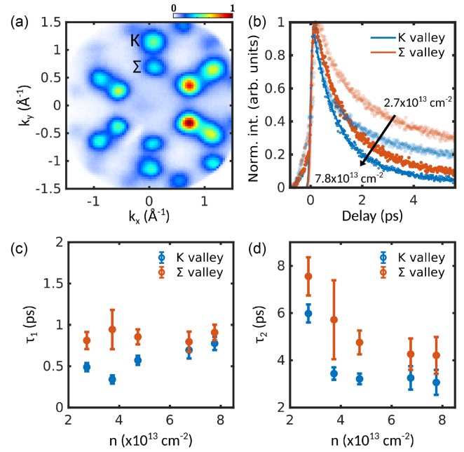
FIG. 3. Photoexcited carrier density-dependent valley-resolved population lifetimes (a) Constant energy contour of excited states near the conduction band minima at the K and \Sigma valleys. The forward-backward asymmetry in photoemission intensity arises from the photoemission transition dipole matrix elements. (b) Time-resolved population dynamics in the K (blue) and \Sigma (red) conduction band valleys for two photoexcited carrier densities ( 2.7 \times 10^{13} \text{ cm}^{-2} and 7.8 \times 10^{13} \text{ cm}^{-2} ). (c), (d) Valley-resolved photoexcited carrier density-dependent time constants ( \tau_1 and \tau_2 , respectively).
