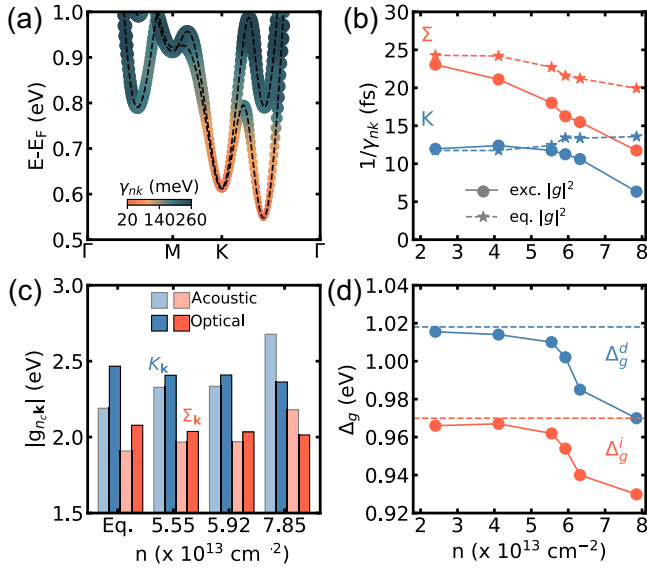
FIG. 4. Equilibrium and nonequilibrium electronic properties of bilayer 2H-MoTe 2 . (a) Band-projected electron linewidth ( \gamma_{nk} ) for conduction bands of bilayer 2H-MoTe 2 along the \Gamma -M-K- \Gamma path. (b) Single-particle electron lifetimes ( 1/\gamma_{nk} ) for various photoexcited carrier densities. The stars and dashed lines represent results obtained using equilibrium EPC matrix elements (eq. |g|^2 ), while the filled circles and full lines show results of cDFPT calculations (including screening of EPC matrix elements by photoexcited carriers, exc. |g|^2 ). (c) Equilibrium and nonequilibrium EPC matrix elements ( |g_{q,\nu}| ) at the bottom of the K (blue) and \Sigma (red) valleys, separated in their acoustic (faint colors) and optical (bold colors) phonon contributions. (d) Direct ( \Delta_g^d , blue) and indirect ( \Delta_g^i , red) band gaps as a function of photoexcited carrier density. The dashed horizontal lines represent the associated band-gap values for which no photoexcited carrier screening of |g|^2 is considered.
