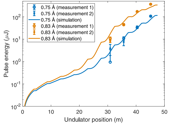
FIG. 4. Measured and simulated FEL gain curves for radiation wavelengths of 0.75 Å and 0.83 Å.
