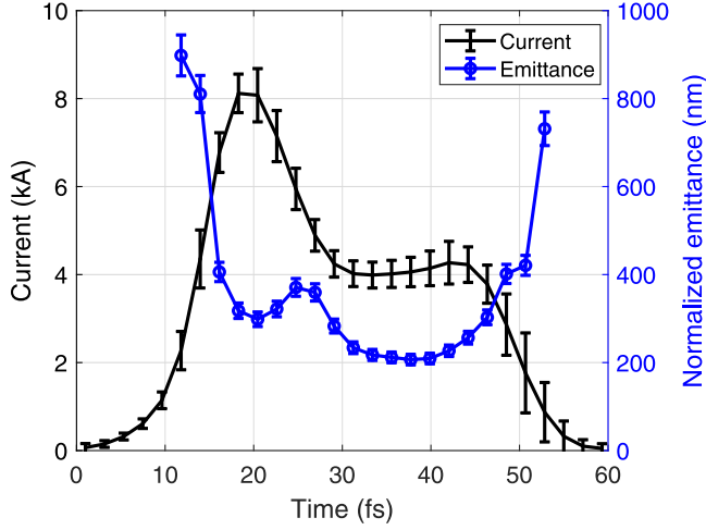
FIG. 3. Current profile and slice emittance measurement of the electron beam.
