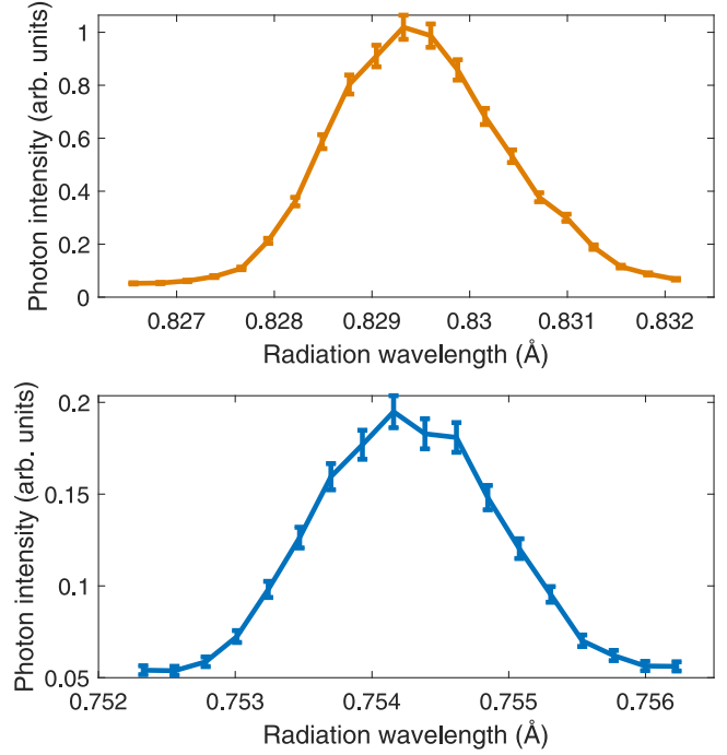
FIG. 2. Spectral measurements for radiation wavelengths of 0.83 Å (top) and 0.75 Å (bottom).
