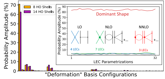
FIG. 2. Probability amplitudes of the “deformation” basis configurations of the {}^6\text{Li} 1_{\text{g.s.}} ground state calculated with NNLO opt in complete model spaces of 8 (yellow) and 14 (purple) HO shells (shown are contributions with probability amplitude \geq 0.1\% ). Inset: The four nuclear shapes with the largest probability amplitudes in the 8-shell {}^6\text{Li} 1_{\text{g.s.}} state across 32 NN parametrizations uniformly sampled within \pm 10\% around the 14 NNLO opt coupling constants (see text for details; cf. Supplemental Material, Fig. 1 [34] for the {}^6\text{Li} 3_1^+ state). While not shown, the inset results remain practically unchanged for 1%–50% LEC variations [42]. Also shown are the Feynman diagrams for chiral NN forces up to NNLO with the total number of LECs per order.
