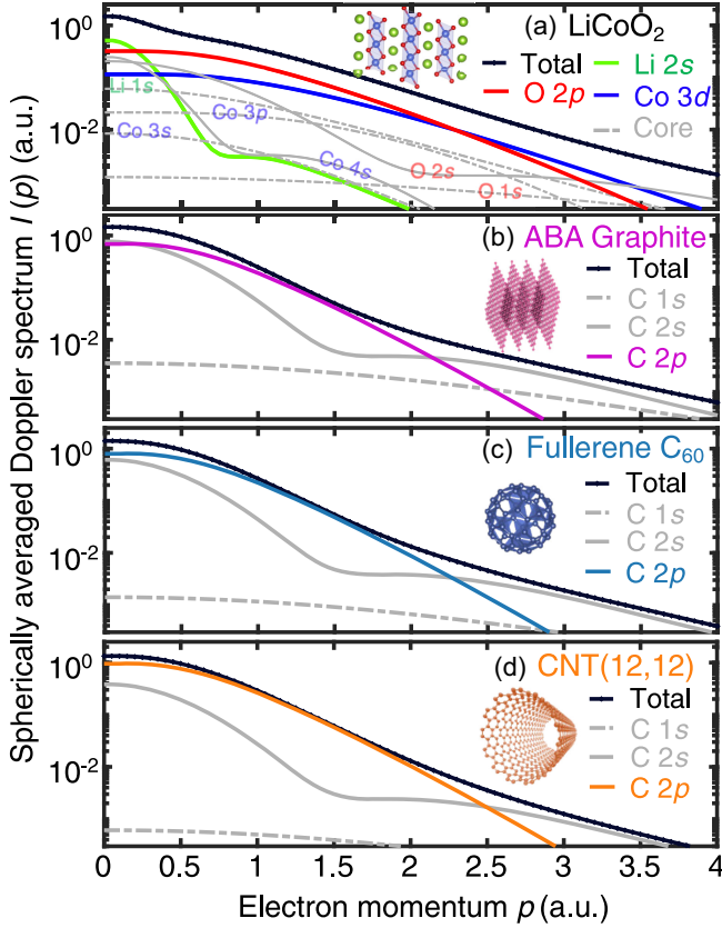
FIG. 2. Calculated spherically averaged Doppler broadening spectrum I(p) of the studied cathode material \text{LiCoO}_2 and carbon coating materials: (a) \text{LiCoO}_2 , (b) ABA Graphite, (c) fullerene \text{C}_{60} and (d) \text{CNT}(12,12) . Distribution of I(p) as a function of the electron-positron annihilation pair's momentum p . Black lines indicate the total spectra, gray dashed lines indicate the core orbital contribution. Key valence orbitals are highlighted using color coding. Results show that positron, as a quantum probe, is particularly sensitive to valence orbitals, traversing in interstitial regions until trapping or annihilation.
