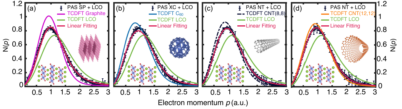
FIG. 3. Momentum distribution, N(p) for calculated LCO and carbon, along with their linear combination, compared with experimental results from diverse samples. The PAS experimental momentum profiles for different samples in (a) super P—SP, (b) carbon nanospheres—XC, and (c),(d) carbon nanotubes—NT, are represented by black lines. The TCDFT calculated momentum distributions for LCO, graphite, C_{60} , CNT(8,8), and CNT(12,12) are color coded by green, magenta, blue, black (dashed), and orange lines, respectively. The theoretical linear combinations of the calculated spectra, as denoted by Eq. (2), are shown in red lines. These profiles are instrumental in identifying the high-momentum electron contributions, serving as a chemical fingerprint of the annihilation sites. The experimental data are derived from our previous work [8]. The distribution N(p) is normalized to one.
