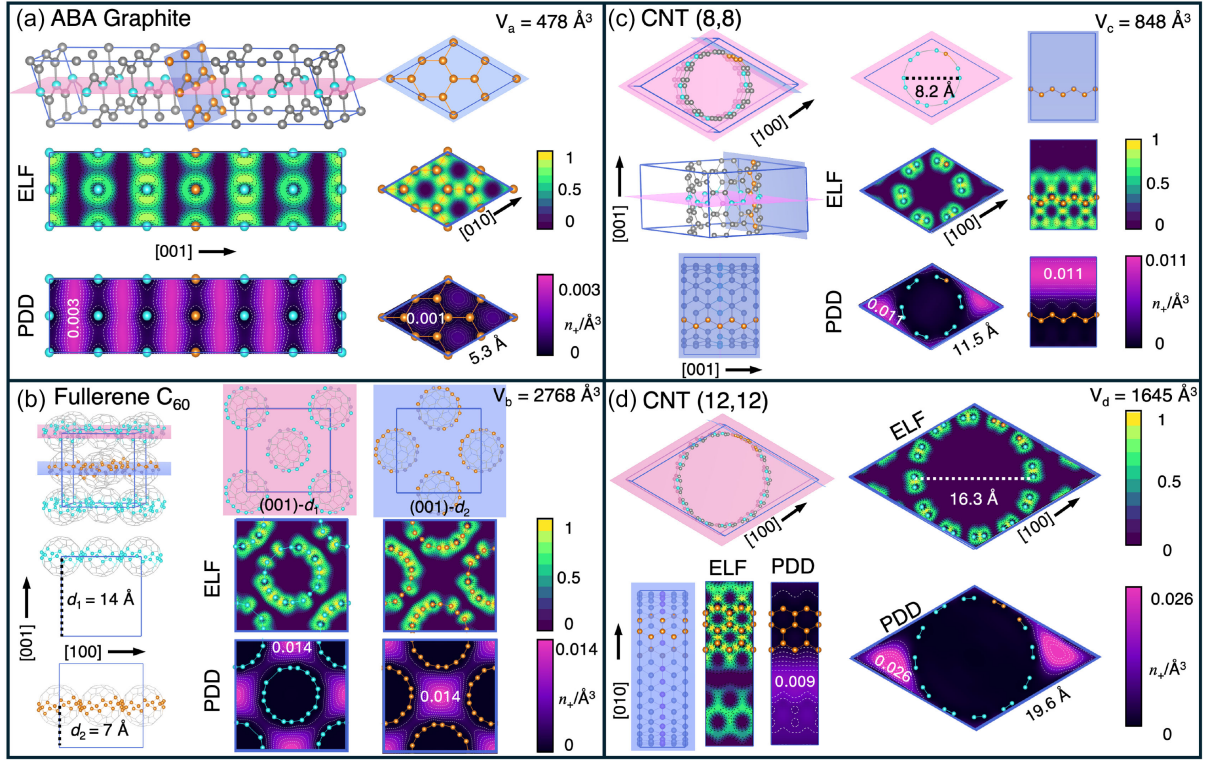
FIG. 1. Calculations of the electron localization function (ELF) and positron density distribution (PDD) n_+(\mathbf{r}) in various carbon allotropes: (a) ABA graphite, (b) fullerene C_{60} , (c) carbon nanotubes CNT(8,8), and (d) CNT(12,12). We selected two distinct planes, represented by pink and blue, to display the results. Carbon atoms are denoted by cyan on the pink plane and by orange on the blue plane. Other carbon atoms are shown in gray. In C_{60} , the planes at different distances along the [001] direction are distinguished as (001)- d_1 and (001)- d_2 . In CNTs, the blue plane reveals the bonding characteristics between conjugated carbon atoms, depicted as an orange chain. Density values reported herein are specific to each system and should not be directly compared, as they are influenced by the chosen packing density and normalization volume. Note the value of n_+(\mathbf{r}) depends on the periodic boundary conditions defined for the unit cells. The optimized six-layer ABA graphite was calculated with an in-plane lattice parameter of a = 5.3 Å and interlayer distance of 3.3 Å. C_{60} exhibits a cubic structure with a parameter a = 14.0 Å. In the case of carbon nanotubes, CNT(8,8) and CNT(12,12) possess diameters of 8.2 and 16.3 Å, respectively.
