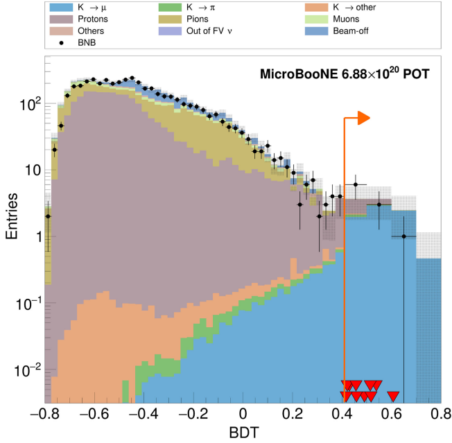
FIG. 2. BDT classifier score distribution. The black dots represent the MicroBooNE data. The stacked histogram represents the expected BDT distribution from the simulation with its statistical uncertainty (gray band). The orange arrow represents the BDT event selection cut. The red triangles are the K^+ candidates selected in MicroBooNE data by the BDT.
