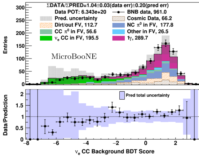
FIG. 1. Distribution of \nu_e CC background rejection BDT scores. This BDT targets the separation of CC events with a true electron shower (green) from single-photon signal events (pink) by focusing on the calorimetry of the start of the shower ( dE/dx ) and shower conversion distances.
