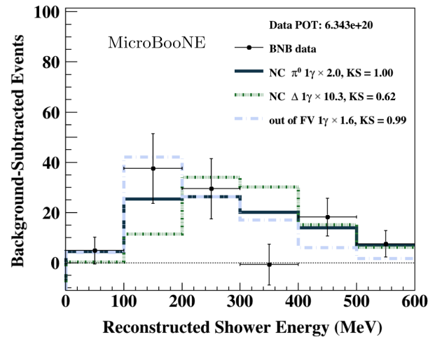
FIG. 5. Shape-only fit for 1\gamma 0p background-subtracted events (data minus constrained prediction). Three signal categories are shown alongside the best fit scaling parameter and the Kolmogorov-Smirnov test statistic. No constraint or systematic uncertainties on the shape of the individual predicted signal categories are considered. The error bars on the data points include both statistical and constrained systematic errors.
