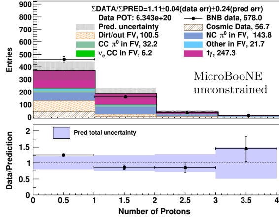
FIG. 3. Numbers of reconstructed primary protons for inclusive single-photon selected events with no constraint applied. The horizontal axis is number of reconstructed protons with kinetic energy above the 35 MeV threshold.
