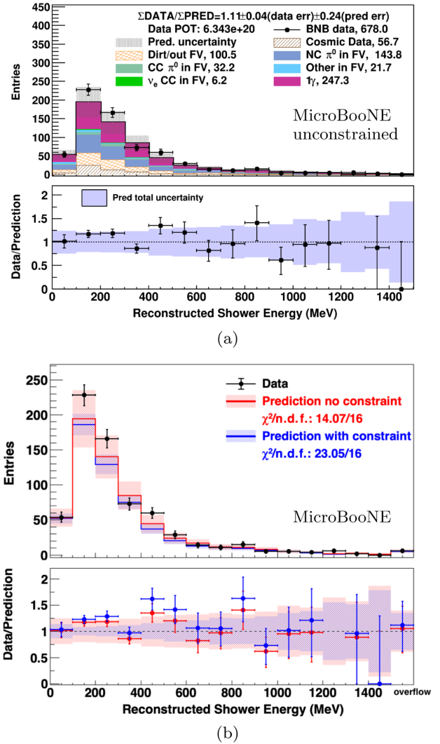
FIG. 2. Reconstructed shower energy for inclusive single-photon selected events, (a) before constraint and (b) before (red) and after (blue) constraint. (a) Shows the inclusive single-photon signal events in pink. The horizontal axis is reconstructed shower energy in 100 MeV bins. Events with energy above 1500 MeV are included via an overflow bin. The constrained prediction has been pulled down in many bins, due to the NC \pi^0 constraining channel predicting more events than seen in the data.
