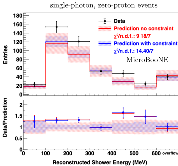
FIG. 4. Reconstructed shower energy for inclusive single-photon, zero-proton selected events, before and after constraint. The horizontal axis is reconstructed shower energy in 100 MeV bins with the last bin containing overflow events.
