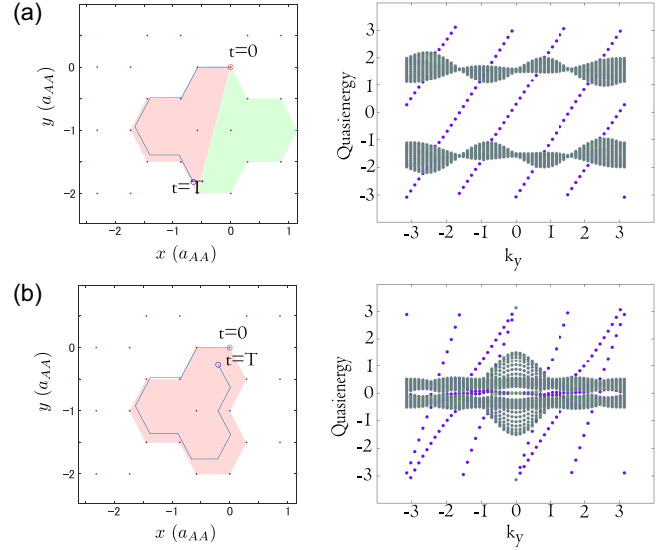
FIG. 3. Protocols for higher winding numbers. (a) Dynamics in the bulk for a protocol where tunneling couplings J_i are alternated according to 1313212. The unit of length is the lattice vector a_{AA} . The driving frequency \omega is chosen to be perfectly resonant, and a deviation from the dispersionless condition is given by a \Delta = 0.221J . The red shading indicates the area enclosed during one Floquet period at the associated dispersionless point. The right panel shows the spectrum in a cylinder geometry with gray color for bulk states and purple color for states residing on one of the edges (the states on the other edge of the system are not shown). The spectrum indicates the winding numbers W_0 = W_\pi = 4 , which matches with the red area A = 2A_u = (W_{0,\pi}/2)A_u . The green shading indicates the area enclosed during the second Floquet period. (b) Same for the driving sequence 131321213232. Here \omega is 0.92 of the resonant value, and \Delta = 0 . While the 0 gap is closed, the spectrum exhibits W_\pi = 2(A/A_u) = 6 and a corresponding red shaded area A = 3A_u = (W_\pi/2)A_u .
