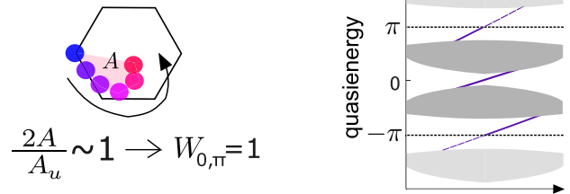
FIG. 1. Bulk observables for Chern systems and anomalous systems. (a) In static systems, the Chern number C determines the number of chiral edge modes (right panel) and can be detected in the bulk by the quantized transverse conductance (left panel). (b) In anomalous Floquet systems, the edge modes are given by the winding numbers W_g for each band gap g . We show that—in the case of dispersionless micromotion dynamics—the micromotion area A is also quantized and indicates the winding numbers while in the more general case, a finite micromotion area can be used to infer the presence of the anomalous phase.
