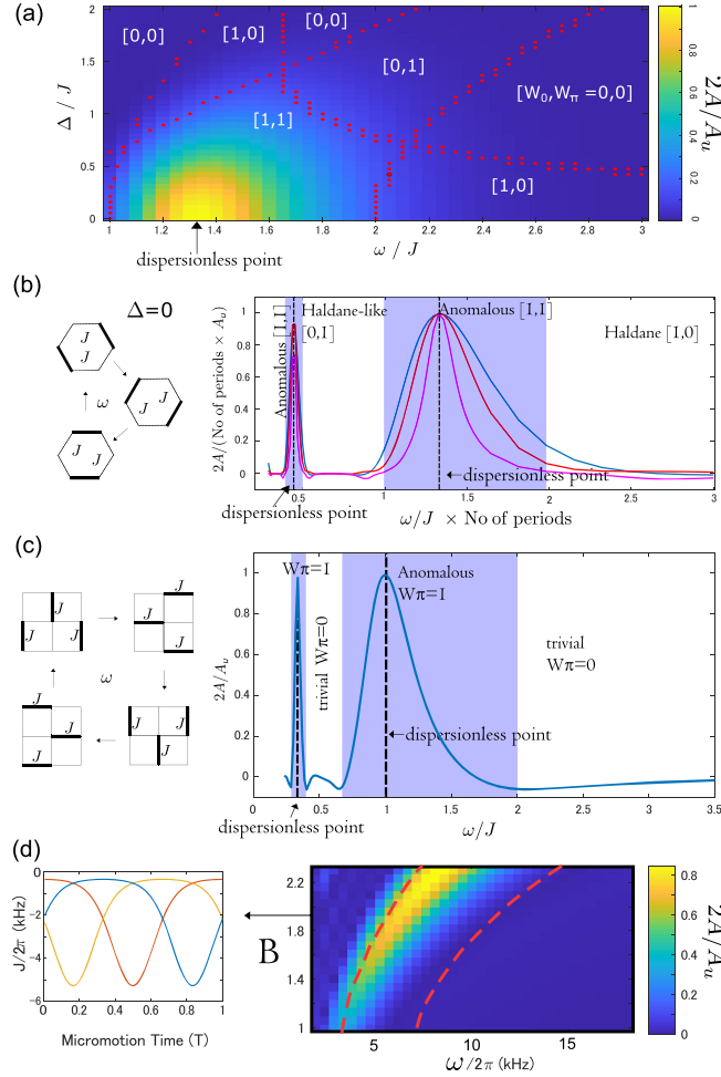
FIG. 2. Micromotion area as a function of \omega and \Delta . (a) Tunneling in a honeycomb lattice is completely switched on and off in a cyclic way J_1 \rightarrow J_2 \rightarrow J_3 \rightarrow \dots with frequency \omega . A constant sublattice offset \Delta is present. We plot the area calculated across the phase diagram. Red dots mark topological phase transition points, and the brackets indicate [W_0, W_\pi] (calculated in [27]). (b) Area (blue curve) as a function of the Floquet frequency for \Delta = 0 . An additional anomalous phase appears for even lower frequency drives [13]. The anomalous phases are indicated by the purple shading. The red (magenta) curve shows the area for two (five) Floquet periods. (c) Area as a function of the Floquet frequency (right) in the cyclic protocol (left) in the bipartite square lattice as introduced in [8]. The 0 gap is always closed for these protocols, and only the value of W_\pi is noted. Also here anomalous phases for smaller driving frequencies are present (purple shading). (d) Micromotion area for a sinusoidal modulation of lattice beam intensities in an optical lattice. The red dashed lines enclose the region of anomalous Floquet topology. Tunnel couplings are modulated as J_n = -p_1 e^{B \cos[2\pi(t/T + n/3)]} + p_2 with p_1/2\pi, p_2/2\pi = 120 \text{ Hz}, -35 \text{ Hz} . The inset shows the time-dependent couplings for B = 1.9 .
