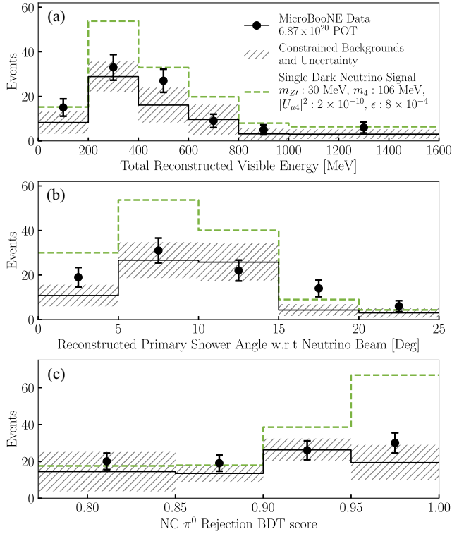
FIG. 3. Final selected data and constrained background prediction for the e^+e^- signal region. Reconstructed total energy (a), the angle that the primary reconstructed shower makes with respect to the incoming neutrino beam (b) and the NC \pi^0 BDT rejection score (c). Shown also in green is a single dark neutrino example signal stacked on top of the background prediction, chosen to lie just within our predicted 95% CL sensitivity, with m_4 = 106 MeV, m_{Z'} = 30 MeV, |U_{\mu 4}|^2 = 2.0 \times 10^{-10} , and \epsilon = 8 \times 10^{-4} . Equivalent spectra for preconstrained backgrounds can be found in Supplemental Material [38].
