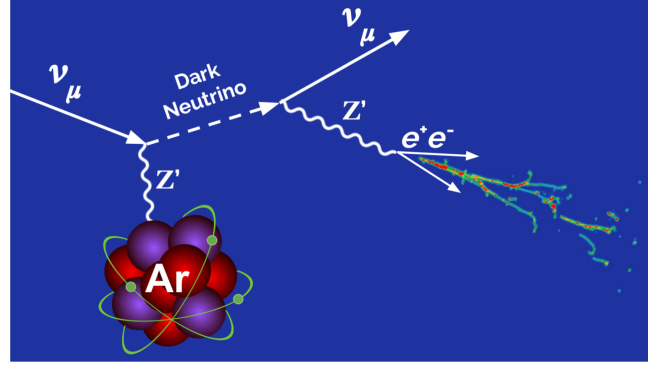
FIG. 1. Example of the dark sector models being probed. An incoming muon-neutrino from the BNB scatters off an argon target producing a dark neutrino. The subsequent decay of the dark neutrino leads to a visible e^+e^- pair, mediated via a new dark gauge boson ( Z' ). A simulated event is also shown behind the e^+e^- arrows to represent what an e^+e^- pair would actually look like in our LArTPC detector after forming electromagnetic showers.
