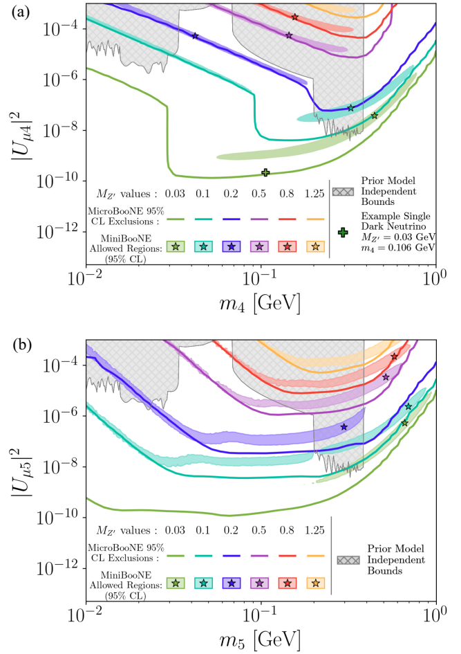
FIG. 4. Resulting MicroBooNE 95% CL exclusion contours for a single dark neutrino model (a) and representative \Delta = 1 dual dark neutrino scenario (b). Each solid line represents MicroBooNE limits for one of six values of the dark gauge boson mass ( m_{Z'} ) varying from 30 MeV to 1.25 GeV, with everything above the solid line being excluded at above the 95% CL. The corresponding MiniBooNE-allowed regions for each dark gauge boson mass indicate the 95% CL preferred region of parameter space that offers a viable explanation to the MiniBooNE anomaly, taken from [37], with each star showing the MiniBooNE best fit for that single value of M_{Z'} . The green plus in (a) indicates the example model point used in Fig. 3. The gray solid regions indicate model-independent limits on dark neutrinos [57–62] prior to this result. The 30 MeV Z' contour in (a) corresponds to the dark neutrino model introduced in Ref. [18]. In both scenarios presented here we fix \epsilon = 8 \times 10^{-4} , g_D = 2 .
